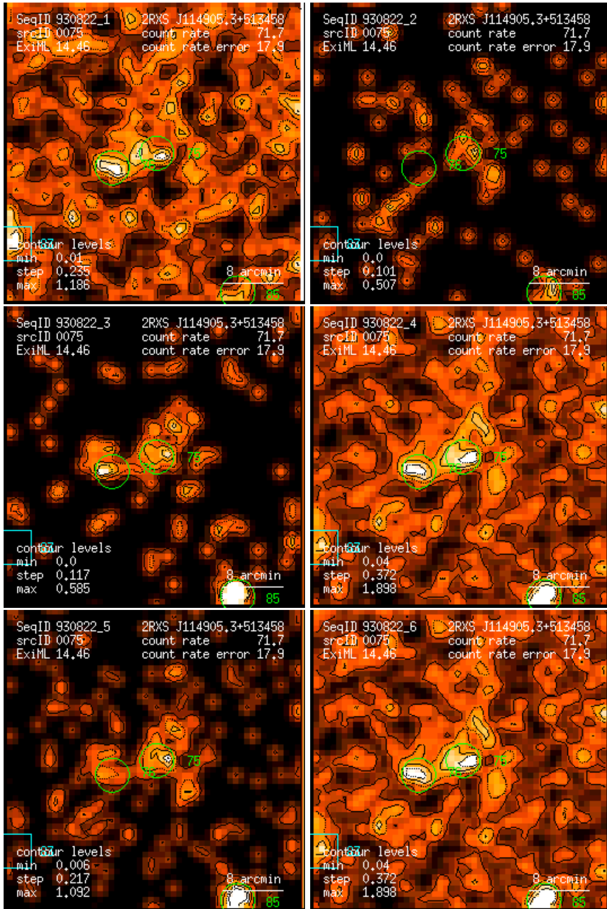
Figure 75: RASS 930822: detection 0075: band rate images, Gaussian filter: (1) PSPC channels 11 – 41, (2) 52 – 90, (3) 91 – 201, (4) 11 – 235, (5) 52 – 201, (6) 11 – 201. Broad band rates in counts/ks. Band rate contour levels in counts/ks/arcmin 2 .
