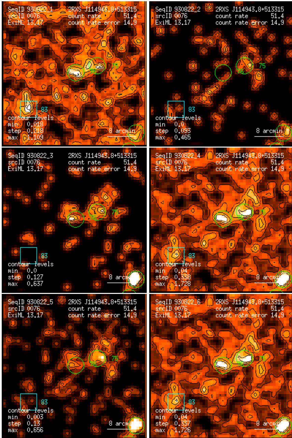
Figure 76: RASS 930822: detection 0076: band rate images, Gaussian filter: (1) PSPC channels 11 – 41, (2) 52 – 90, (3) 91 – 201, (4) 11 – 235, (5) 52 – 201, (6) 11 – 201. Broad band rates in counts/ks. Band rate contour levels in counts/ks/arcmin 2 .
