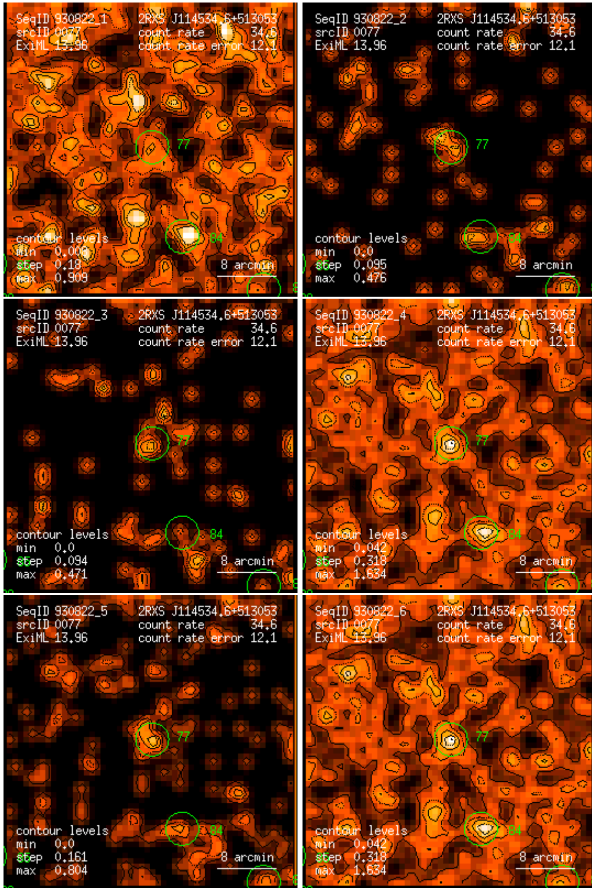
Figure 77: RASS 930822: detection 0077: band rate images, Gaussian filter: (1) PSPC channels 11 – 41, (2) 52 – 90, (3) 91 – 201, (4) 11 – 235, (5) 52 – 201, (6) 11 – 201. Broad band rates in counts/ks. Band rate contour levels in counts/ks/arcmin 2 .
