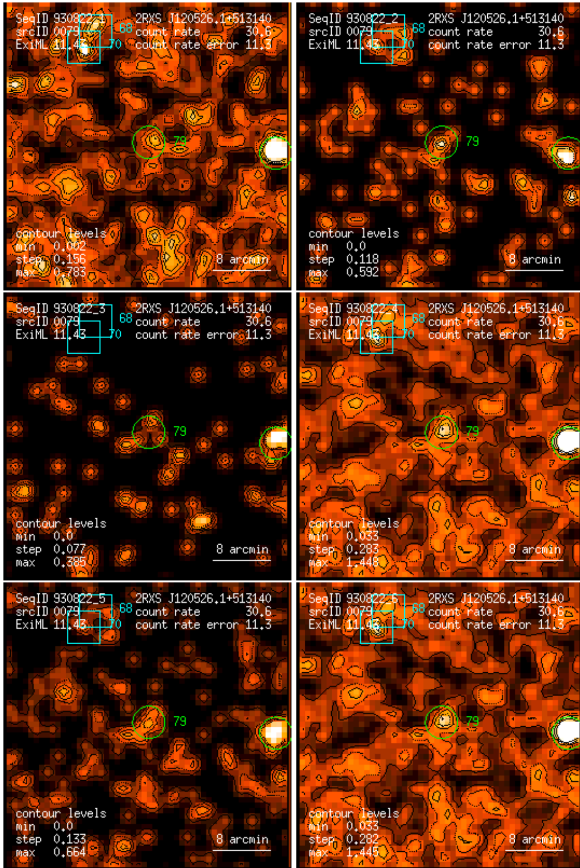
Figure 79: RASS 930822: detection 0079: band rate images, Gaussian filter: (1) PSPC channels 11 – 41, (2) 52 – 90, (3) 91 – 201, (4) 11 – 235, (5) 52 – 201, (6) 11 – 201. Broad band rates in counts/ks. Band rate contour levels in counts/ks/arcmin 2 .
