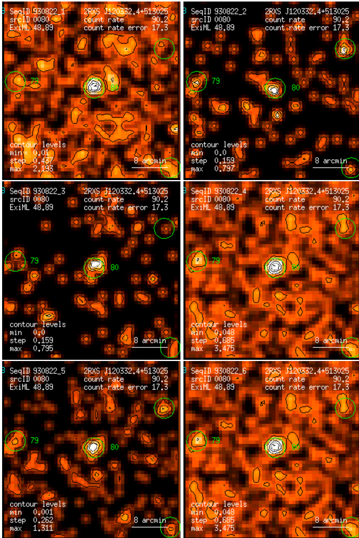
Figure 80: RASS 930822: detection 0080: band rate images, Gaussian filter: (1) PSPC channels 11 – 41, (2) 52 – 90, (3) 91 – 201, (4) 11 – 235, (5) 52 – 201, (6) 11 – 201. Broad band rates in counts/ks. Band rate contour levels in counts/ks/arcmin 2 .
