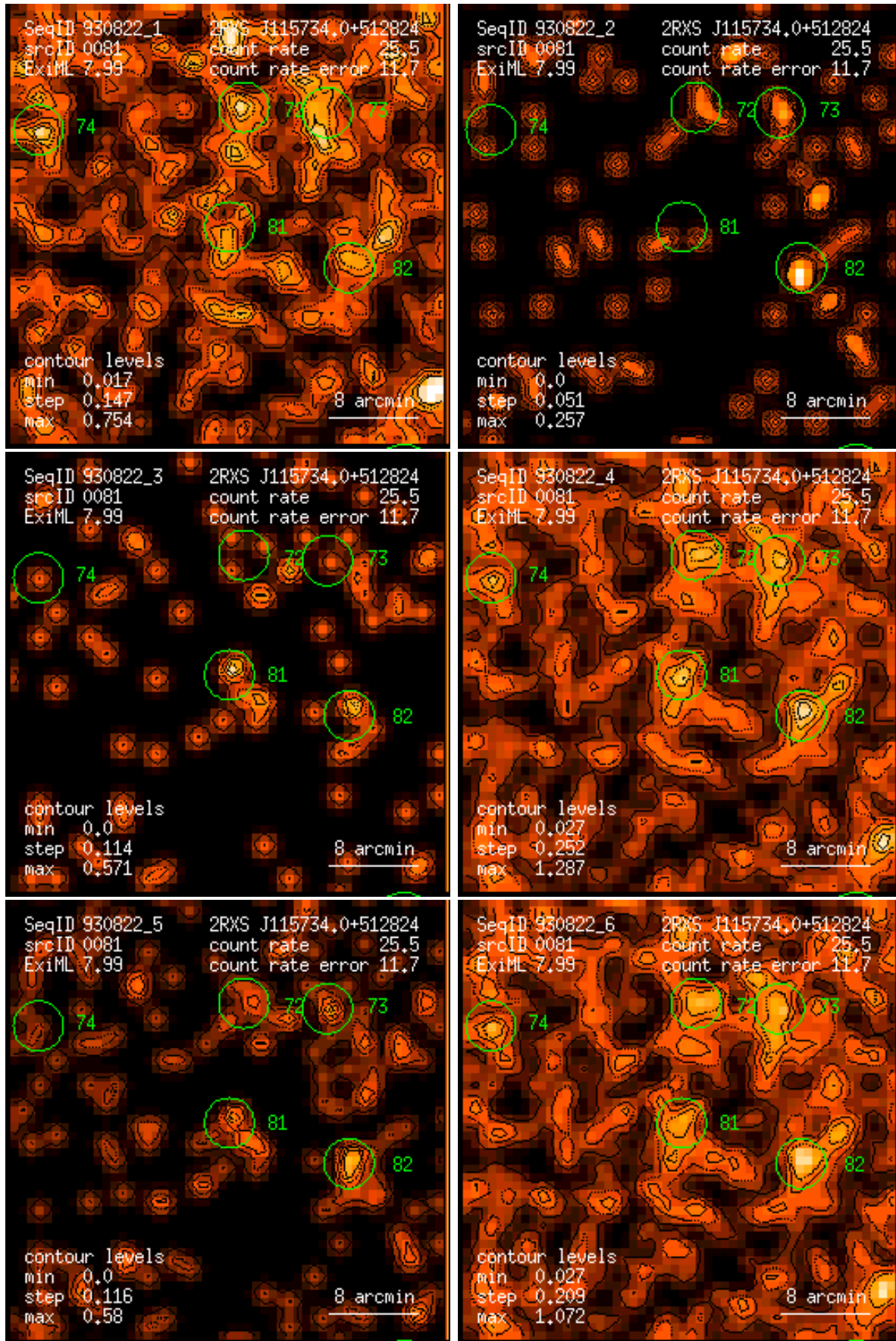
Figure 81: RASS 930822: detection 0081: band rate images, Gaussian filter: (1) PSPC channels 11 – 41, (2) 52 – 90, (3) 91 – 201, (4) 11 – 235, (5) 52 – 201, (6) 11 – 201. Broad band rates in counts/ks. Band rate contour levels in counts/ks/arcmin 2 .
