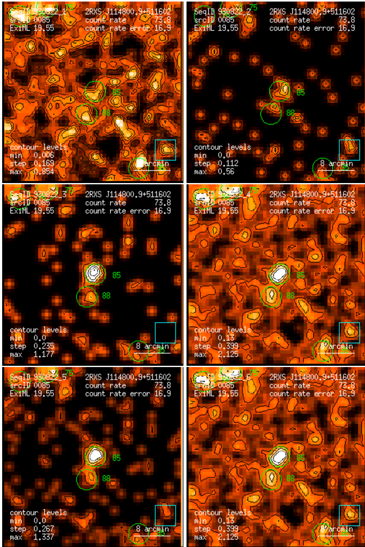
Figure 85: RASS 930822: detection 0085: band rate images, Gaussian filter: (1) PSPC channels 11 – 41, (2) 52 – 90, (3) 91 – 201, (4) 11 – 235, (5) 52 – 201, (6) 11 – 201. Broad band rates in counts/ks. Band rate contour levels in counts/ks/arcmin 2 .
