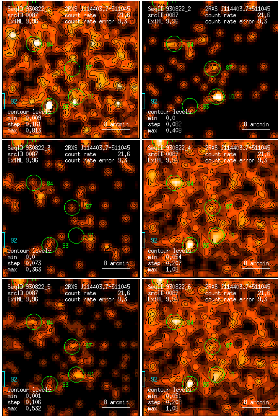
Figure 87: RASS 930822: detection 0087: band rate images, Gaussian filter: (1) PSPC channels 11 – 41, (2) 52 – 90, (3) 91 – 201, (4) 11 – 235, (5) 52 – 201, (6) 11 – 201. Broad band rates in counts/ks. Band rate contour levels in counts/ks/arcmin 2 .
