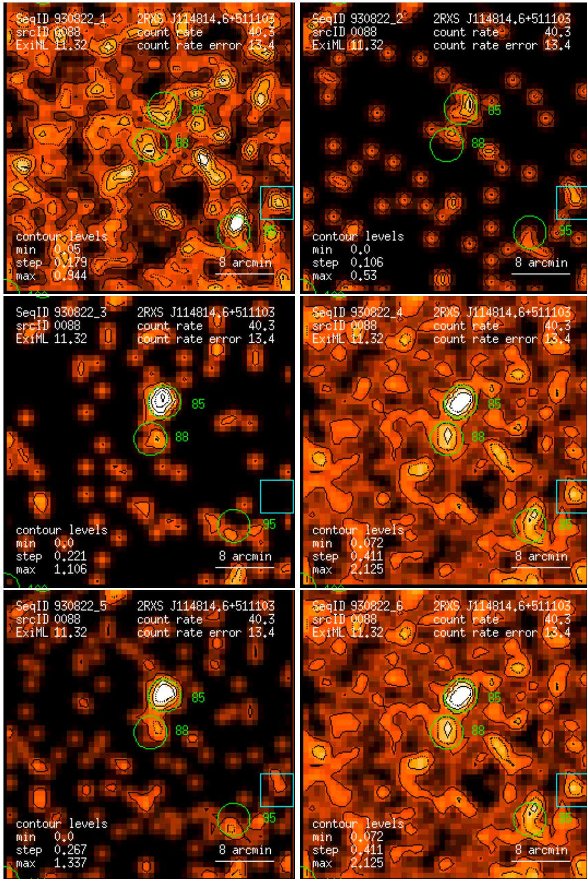
Figure 88: RASS 930822: detection 0088: band rate images, Gaussian filter: (1) PSPC channels 11 – 41, (2) 52 – 90, (3) 91 – 201, (4) 11 – 235, (5) 52 – 201, (6) 11 – 201. Broad band rates in counts/ks. Band rate contour levels in counts/ks/arcmin 2 .
