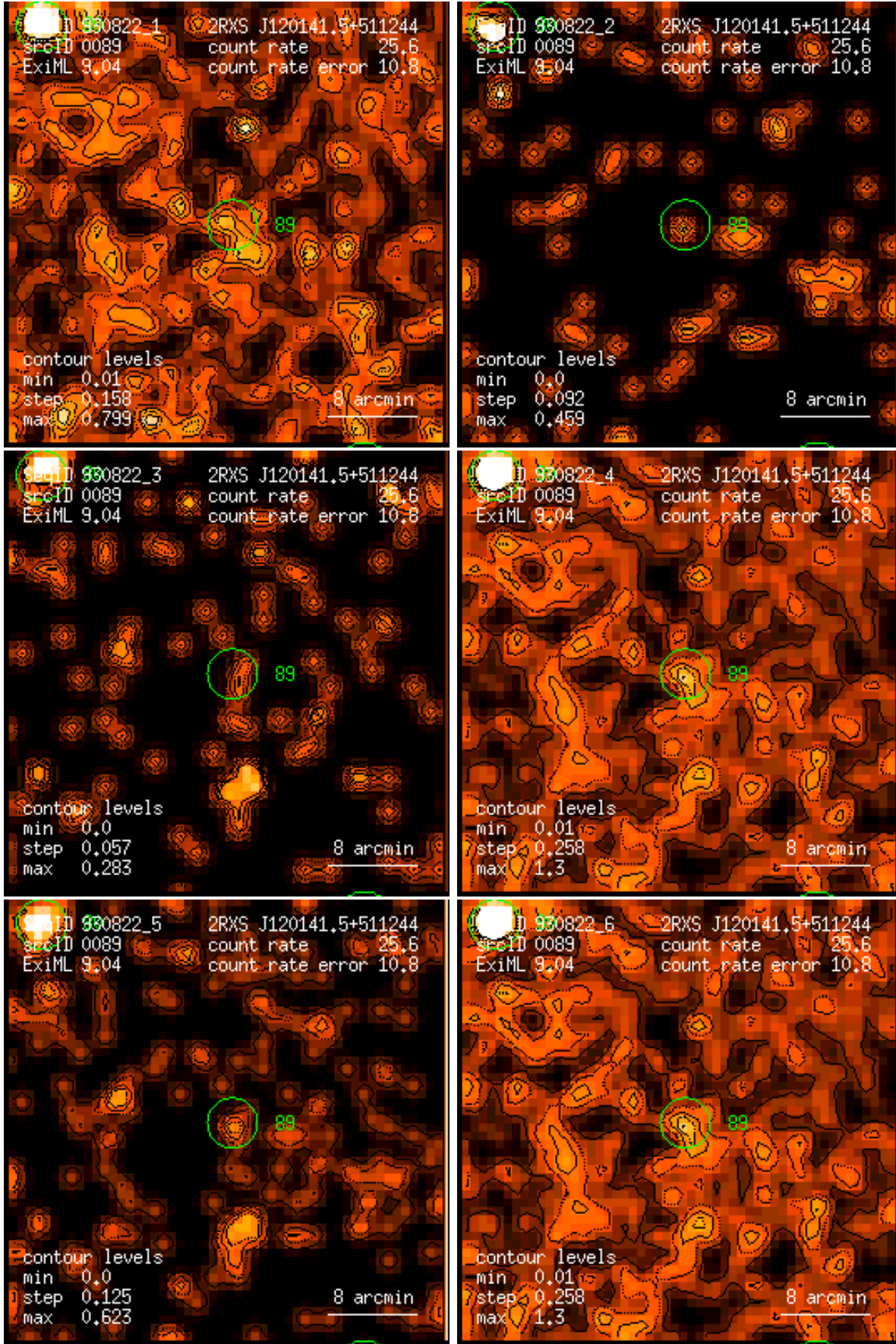
Figure 89: RASS 930822: detection 0089: band rate images, Gaussian filter: (1) PSPC channels 11 – 41, (2) 52 – 90, (3) 91 – 201, (4) 11 – 235, (5) 52 – 201, (6) 11 – 201. Broad band rates in counts/ks. Band rate contour levels in counts/ks/arcmin 2 .
