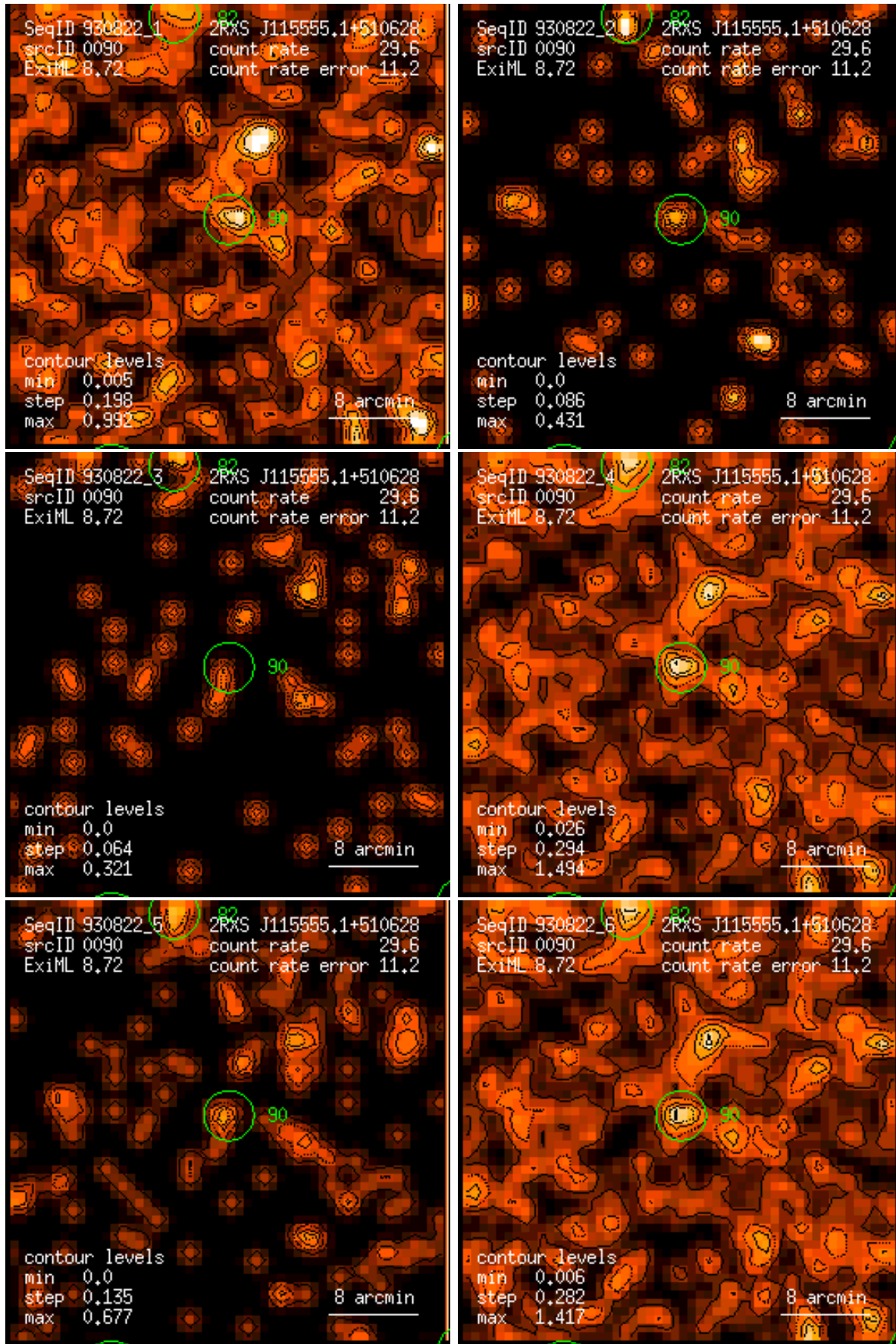
Figure 90: RASS 930822: detection 0090: band rate images, Gaussian filter: (1) PSPC channels 11 – 41, (2) 52 – 90, (3) 91 – 201, (4) 11 – 235, (5) 52 – 201, (6) 11 – 201. Broad band rates in counts/ks. Band rate contour levels in counts/ks/arcmin 2 .
