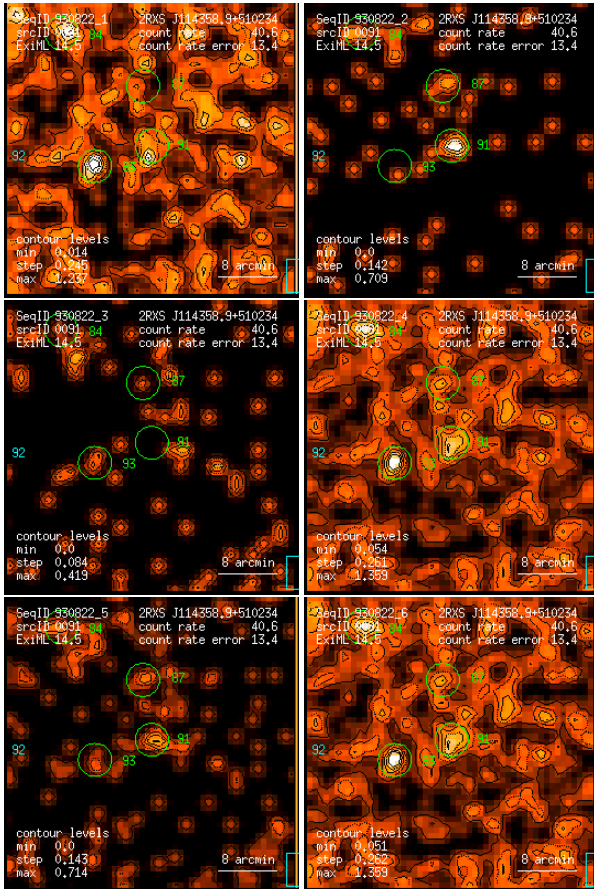
Figure 91: RASS 930822: detection 0091: band rate images, Gaussian filter: (1) PSPC channels 11 – 41, (2) 52 – 90, (3) 91 – 201, (4) 11 – 235, (5) 52 – 201, (6) 11 – 201. Broad band rates in counts/ks. Band rate contour levels in counts/ks/arcmin 2 .
