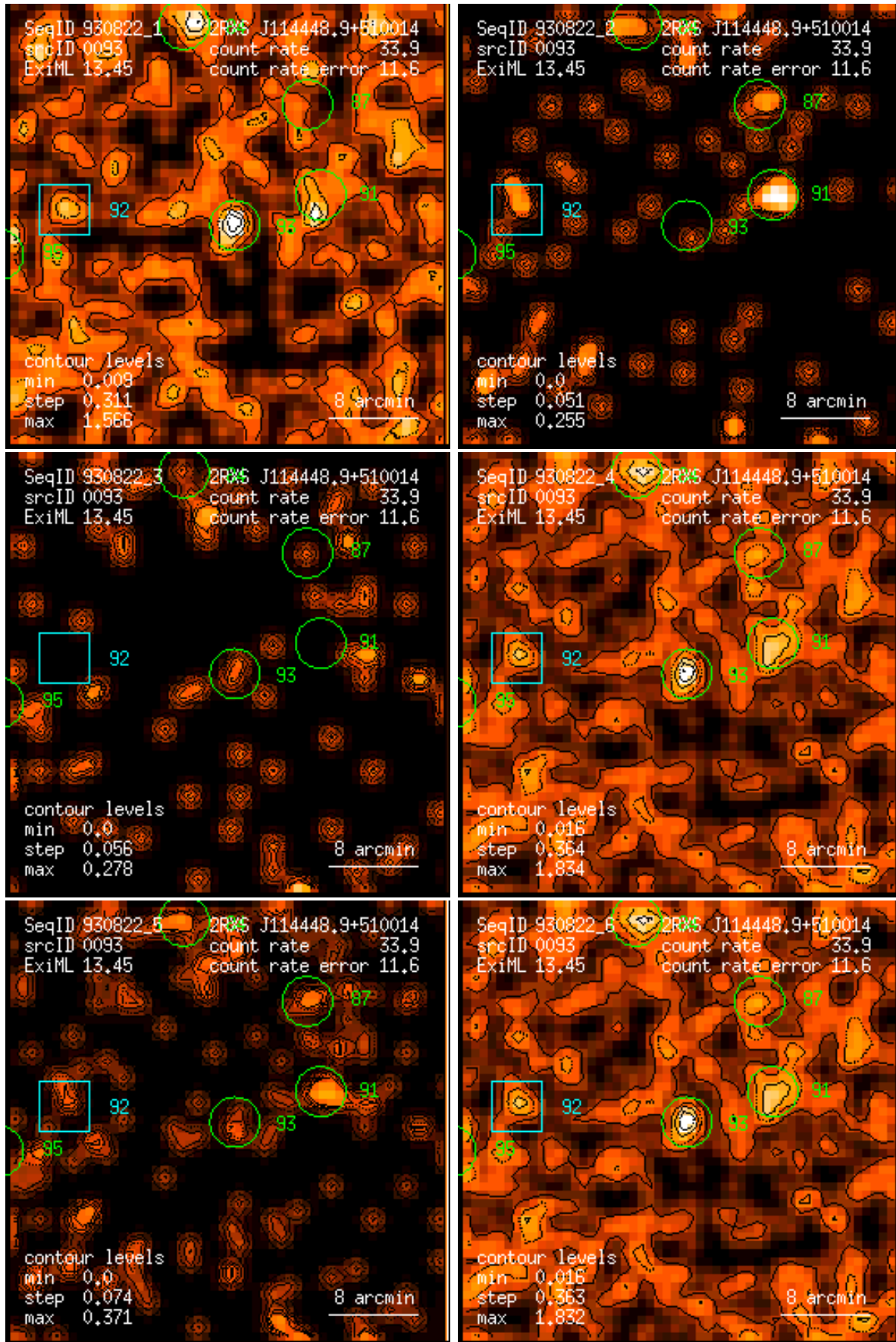
Figure 93: RASS 930822: detection 0093: band rate images, Gaussian filter: (1) PSPC channels 11 – 41, (2) 52 – 90, (3) 91 – 201, (4) 11 – 235, (5) 52 – 201, (6) 11 – 201. Broad band rates in counts/ks. Band rate contour levels in counts/ks/arcmin 2 .
