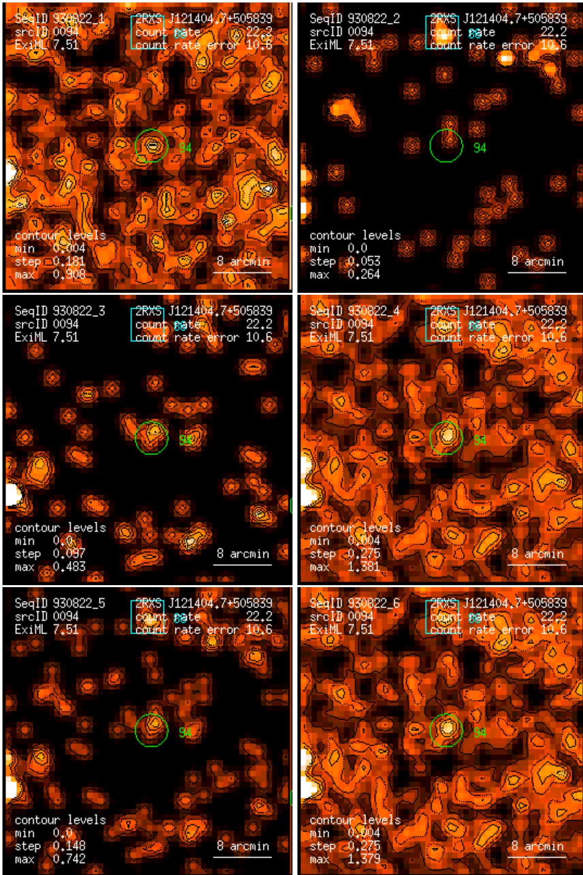
Figure 94: RASS 930822: detection 0094: band rate images, Gaussian filter: (1) PSPC channels 11 – 41, (2) 52 – 90, (3) 91 – 201, (4) 11 – 235, (5) 52 – 201, (6) 11 – 201. Broad band rates in counts/ks. Band rate contour levels in counts/ks/arcmin 2 .
