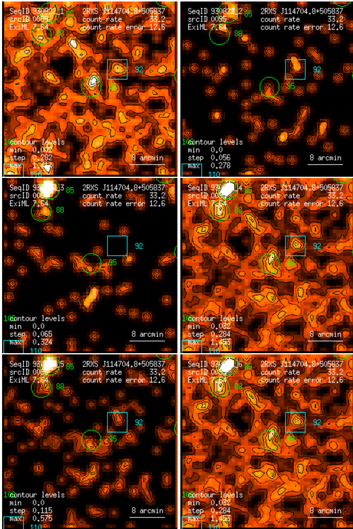
Figure 95: RASS 930822: detection 0095: band rate images, Gaussian filter: (1) PSPC channels 11 – 41, (2) 52 – 90, (3) 91 – 201, (4) 11 – 235, (5) 52 – 201, (6) 11 – 201. Broad band rates in counts/ks. Band rate contour levels in counts/ks/arcmin 2 .
