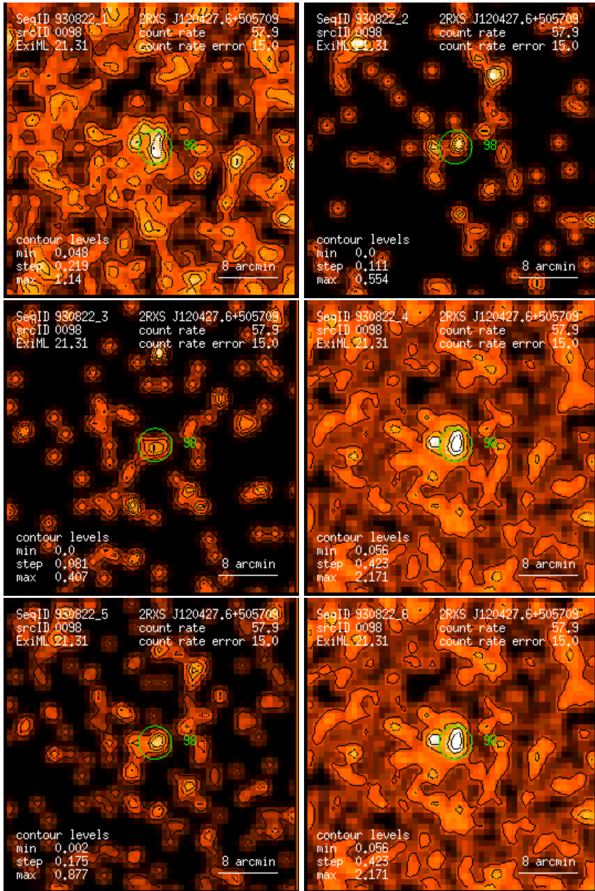
Figure 98: RASS 930822: detection 0098: band rate images, Gaussian filter: (1) PSPC channels 11 – 41, (2) 52 – 90, (3) 91 – 201, (4) 11 – 235, (5) 52 – 201, (6) 11 – 201. Broad band rates in counts/ks. Band rate contour levels in counts/ks/arcmin 2 .
