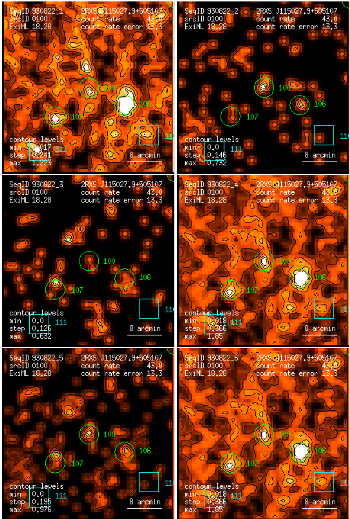
Figure 100: RASS 930822: detection 0100: band rate images, Gaussian filter: (1) PSPC channels 11 – 41, (2) 52 – 90, (3) 91 – 201, (4) 11 – 235, (5) 52 – 201, (6) 11 – 201. Broad band rates in counts/ks. Band rate contour levels in counts/ks/arcmin 2 .
