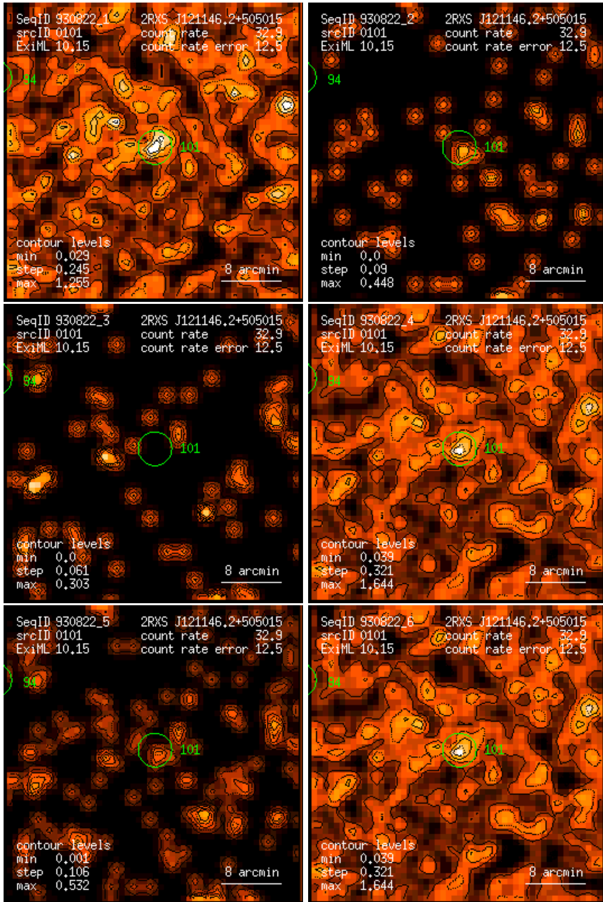
Figure 101: RASS 930822: detection 0101: band rate images, Gaussian filter: (1) PSPC channels 11 – 41, (2) 52 – 90, (3) 91 – 201, (4) 11 – 235, (5) 52 – 201, (6) 11 – 201. Broad band rates in counts/ks. Band rate contour levels in counts/ks/arcmin 2 .
