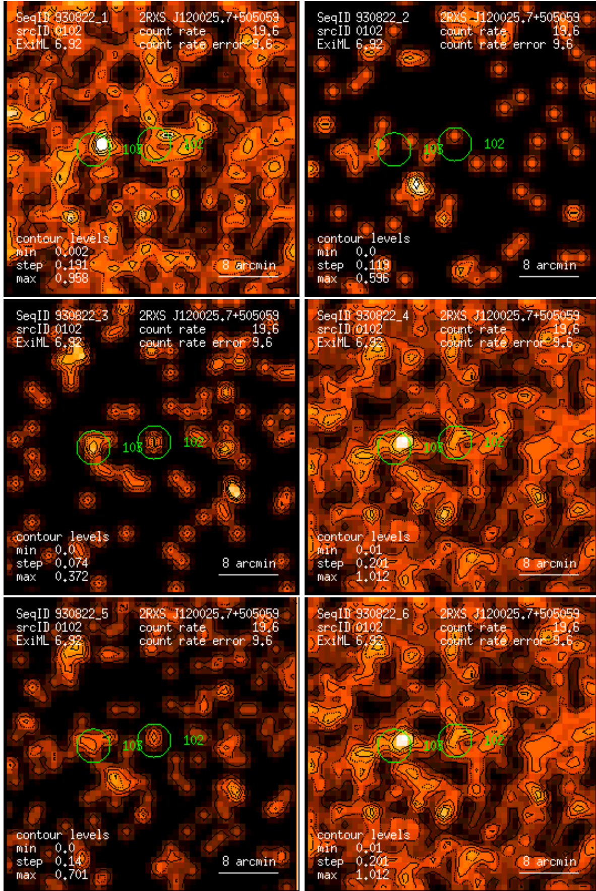
Figure 102: RASS 930822: detection 0102: band rate images, Gaussian filter: (1) PSPC channels 11 – 41, (2) 52 – 90, (3) 91 – 201, (4) 11 – 235, (5) 52 – 201, (6) 11 – 201. Broad band rates in counts/ks. Band rate contour levels in counts/ks/arcmin 2 .
