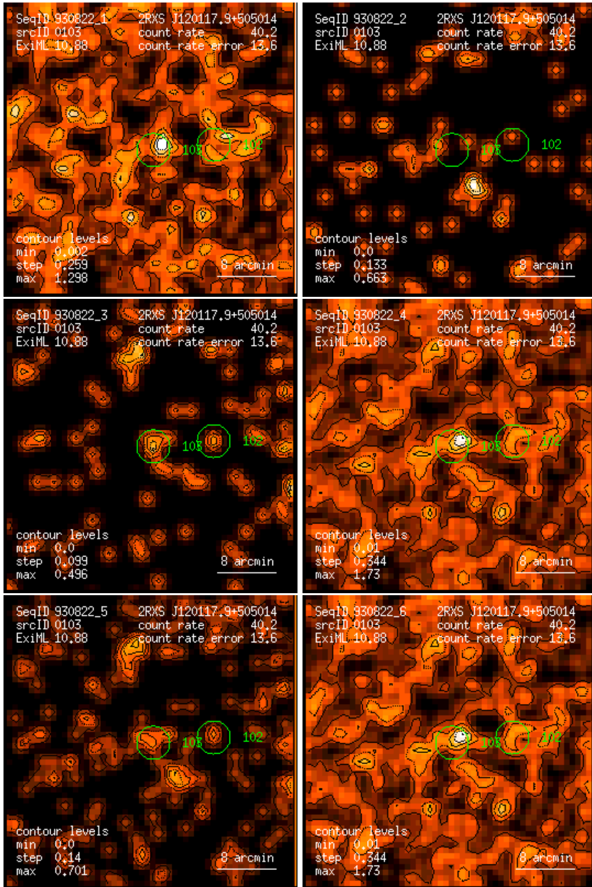
Figure 103: RASS 930822: detection 0103: band rate images, Gaussian filter: (1) PSPC channels 11 – 41, (2) 52 – 90, (3) 91 – 201, (4) 11 – 235, (5) 52 – 201, (6) 11 – 201. Broad band rates in counts/ks. Band rate contour levels in counts/ks/arcmin 2 .
