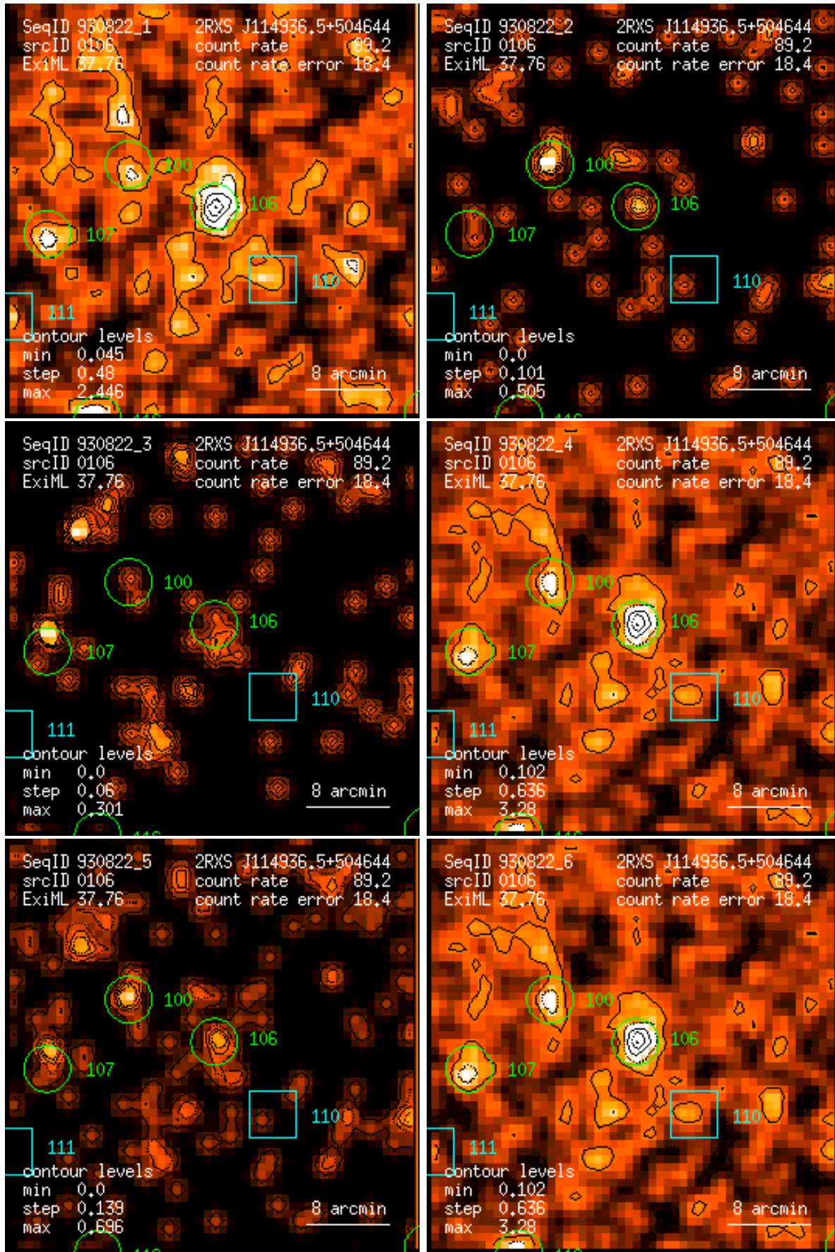
Figure 106: RASS 930822: detection 0106: band rate images, Gaussian filter: (1) PSPC channels 11 – 41, (2) 52 – 90, (3) 91 – 201, (4) 11 – 235, (5) 52 – 201, (6) 11 – 201. Broad band rates in counts/ks. Band rate contour levels in counts/ks/arcmin 2 .
