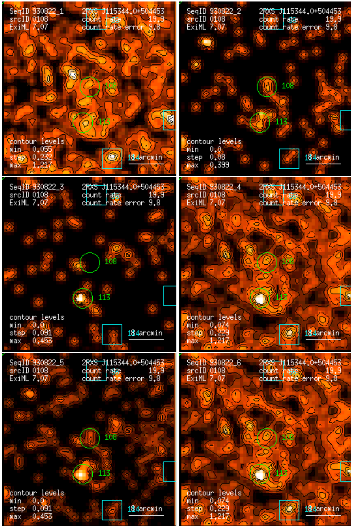
Figure 108: RASS 930822: detection 0108: band rate images, Gaussian filter: (1) PSPC channels 11 – 41, (2) 52 – 90, (3) 91 – 201, (4) 11 – 235, (5) 52 – 201, (6) 11 – 201. Broad band rates in counts/ks. Band rate contour levels in counts/ks/arcmin 2 .
