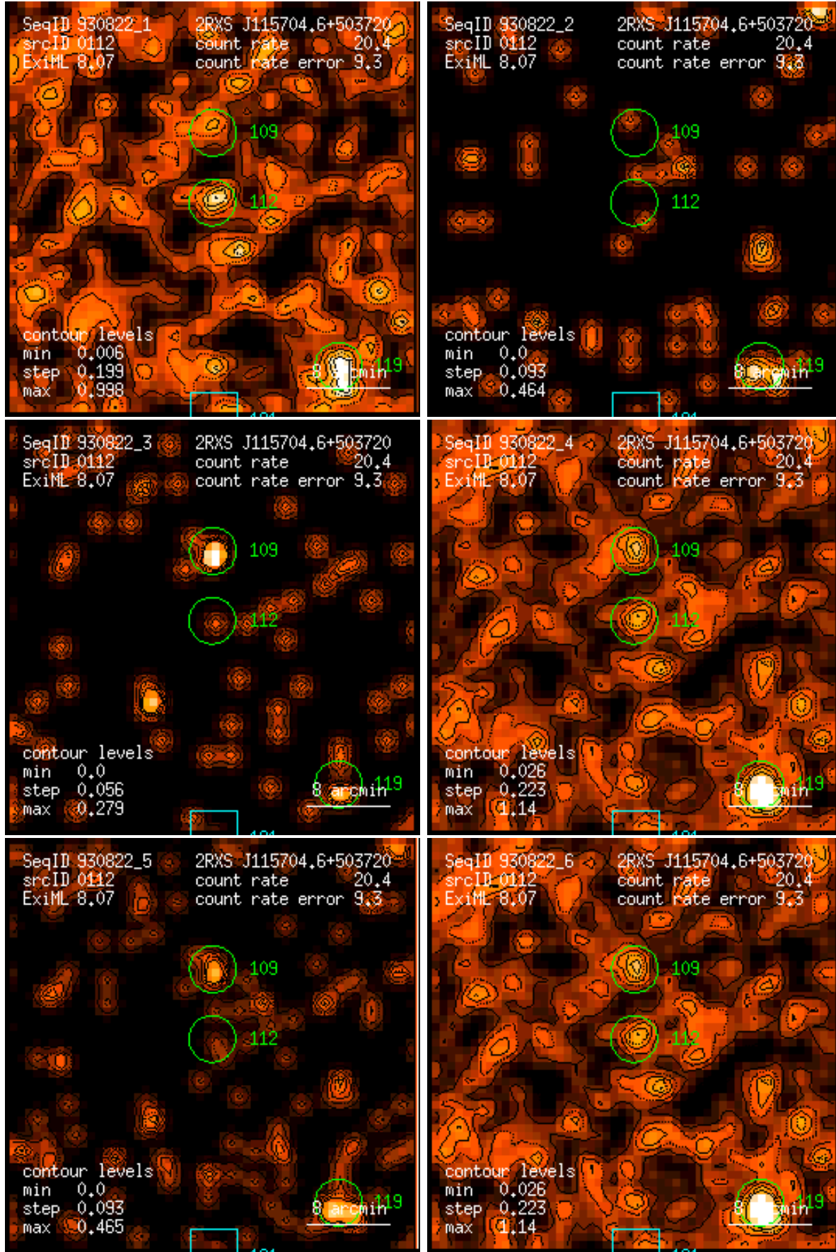
Figure 112: RASS 930822: detection 0112: band rate images, Gaussian filter: (1) PSPC channels 11 – 41, (2) 52 – 90, (3) 91 – 201, (4) 11 – 235, (5) 52 – 201, (6) 11 – 201. Broad band rates in counts/ks. Band rate contour levels in counts/ks/arcmin 2 .
