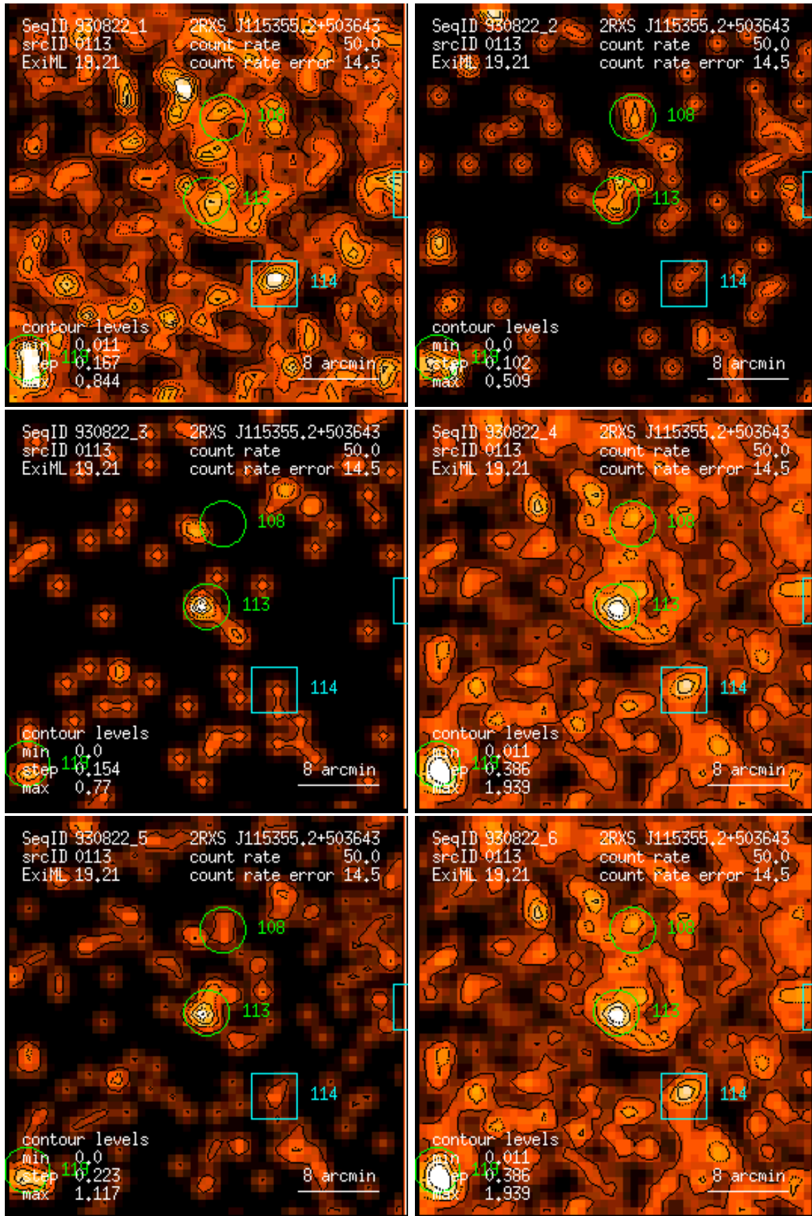
Figure 113: RASS 930822: detection 0113: band rate images, Gaussian filter: (1) PSPC channels 11 – 41, (2) 52 – 90, (3) 91 – 201, (4) 11 – 235, (5) 52 – 201, (6) 11 – 201. Broad band rates in counts/ks. Band rate contour levels in counts/ks/arcmin 2 .
