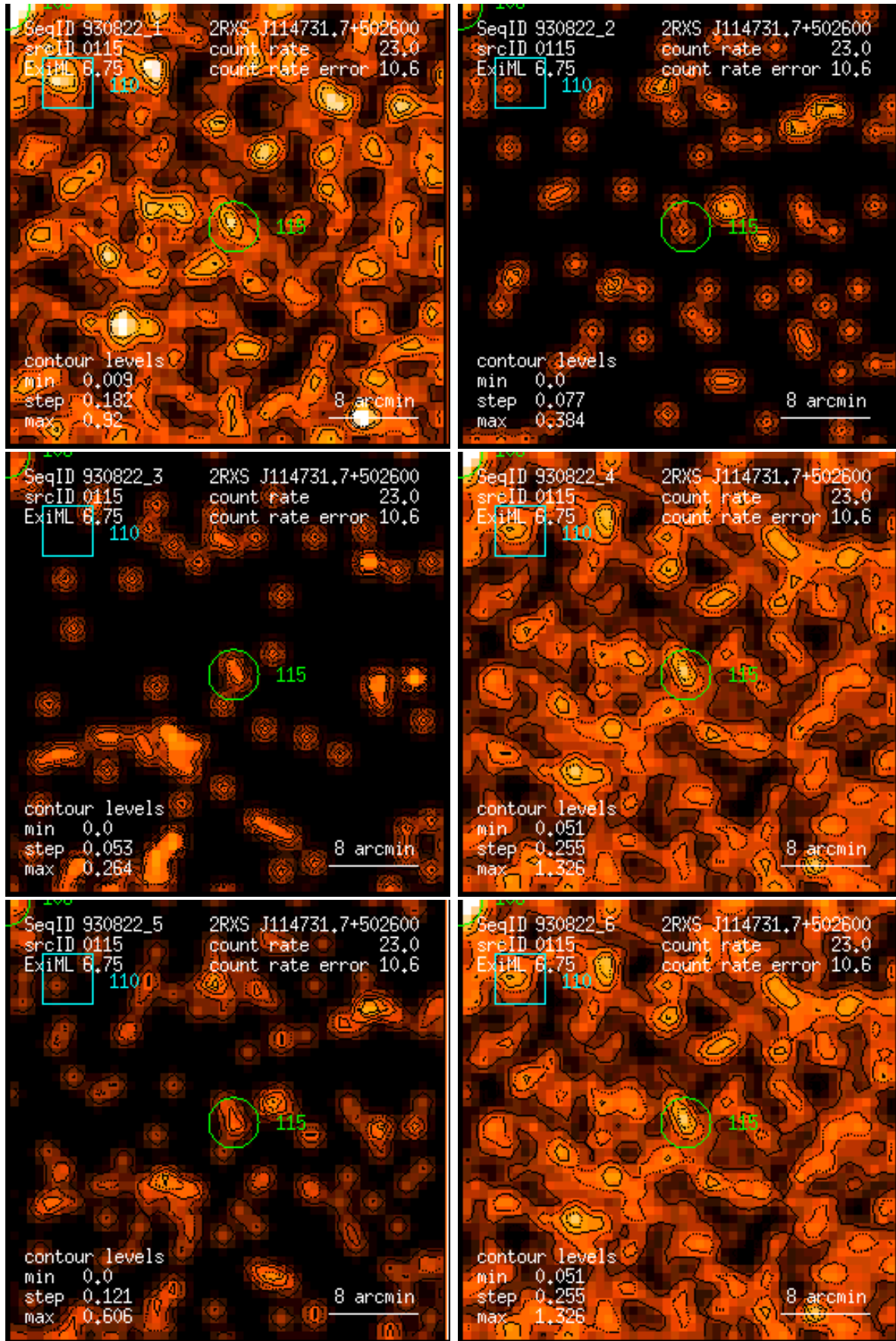
Figure 115: RASS 930822: detection 0115: band rate images, Gaussian filter: (1) PSPC channels 11 – 41, (2) 52 – 90, (3) 91 – 201, (4) 11 – 235, (5) 52 – 201, (6) 11 – 201. Broad band rates in counts/ks. Band rate contour levels in counts/ks/arcmin 2 .
