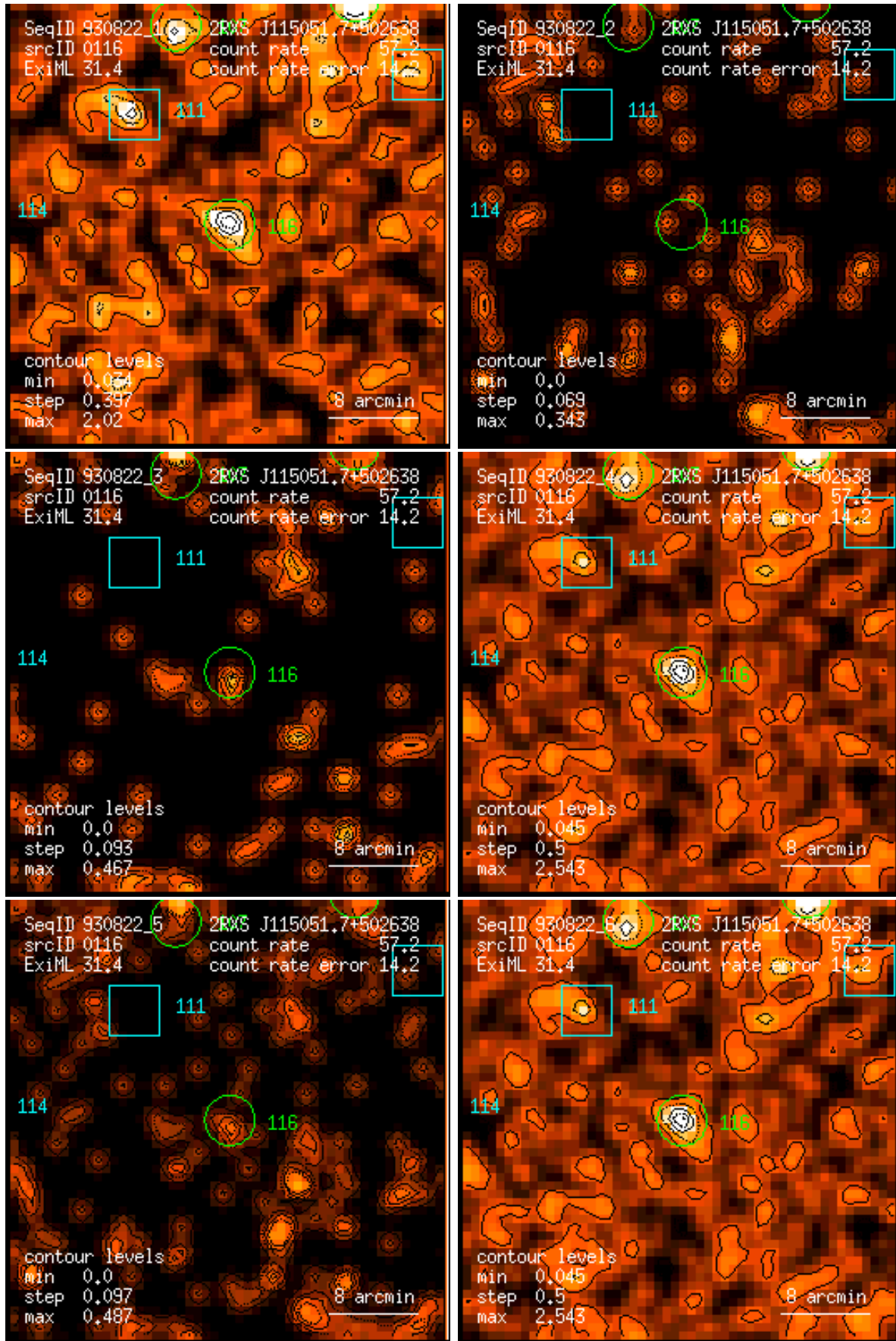
Figure 116: RASS 930822: detection 0116: band rate images, Gaussian filter: (1) PSPC channels 11 – 41, (2) 52 – 90, (3) 91 – 201, (4) 11 – 235, (5) 52 – 201, (6) 11 – 201. Broad band rates in counts/ks. Band rate contour levels in counts/ks/arcmin 2 .
