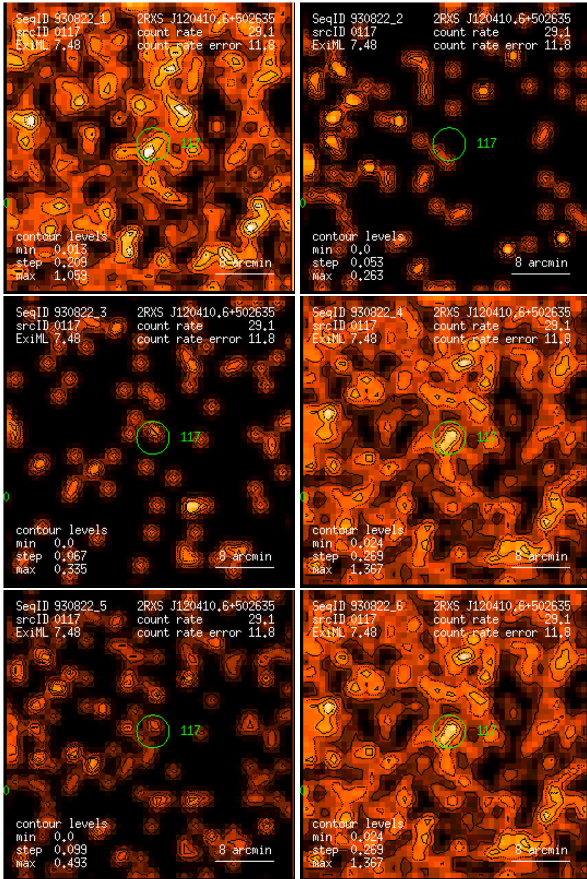
Figure 117: RASS 930822: detection 0117: band rate images, Gaussian filter: (1) PSPC channels 11 – 41, (2) 52 – 90, (3) 91 – 201, (4) 11 – 235, (5) 52 – 201, (6) 11 – 201. Broad band rates in counts/ks. Band rate contour levels in counts/ks/arcmin 2 .
