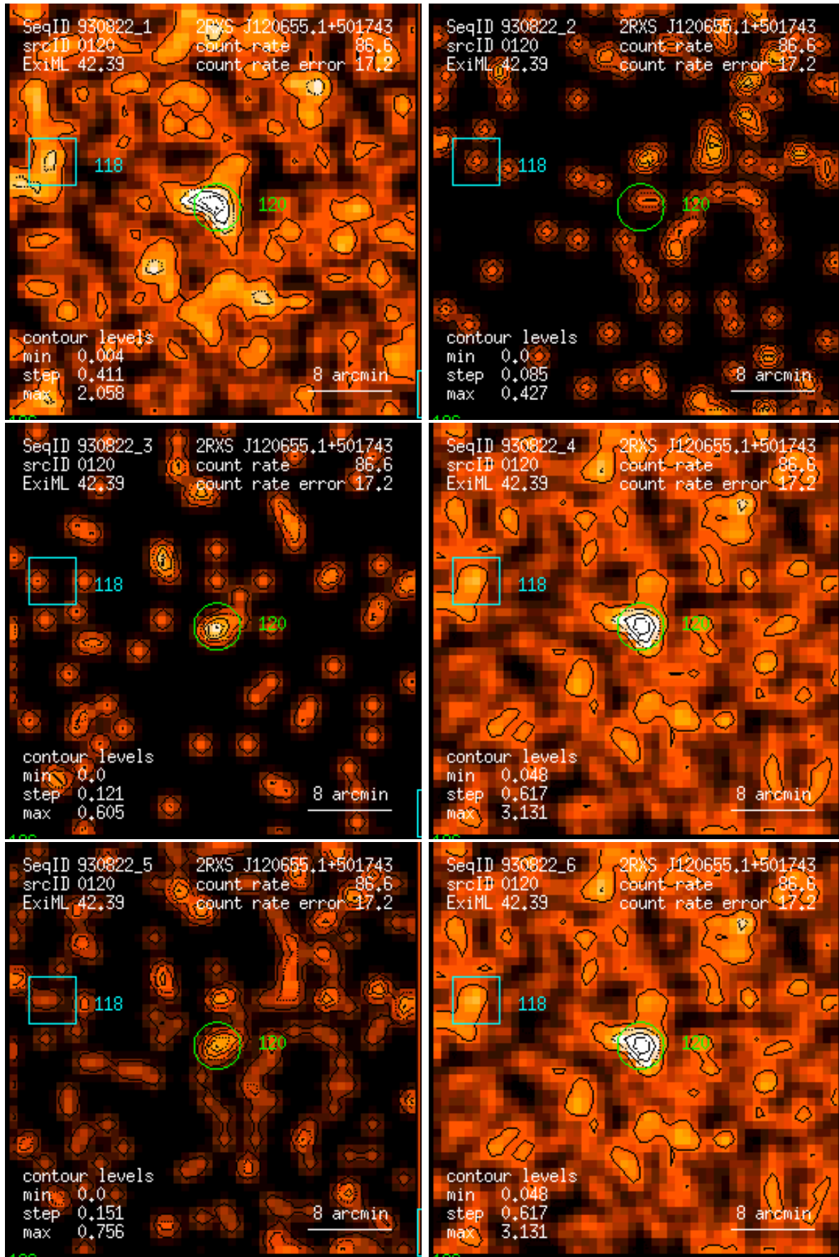
Figure 120: RASS 930822: detection 0120: band rate images, Gaussian filter: (1) PSPC channels 11 – 41, (2) 52 – 90, (3) 91 – 201, (4) 11 – 235, (5) 52 – 201, (6) 11 – 201. Broad band rates in counts/ks. Band rate contour levels in counts/ks/arcmin 2 .
