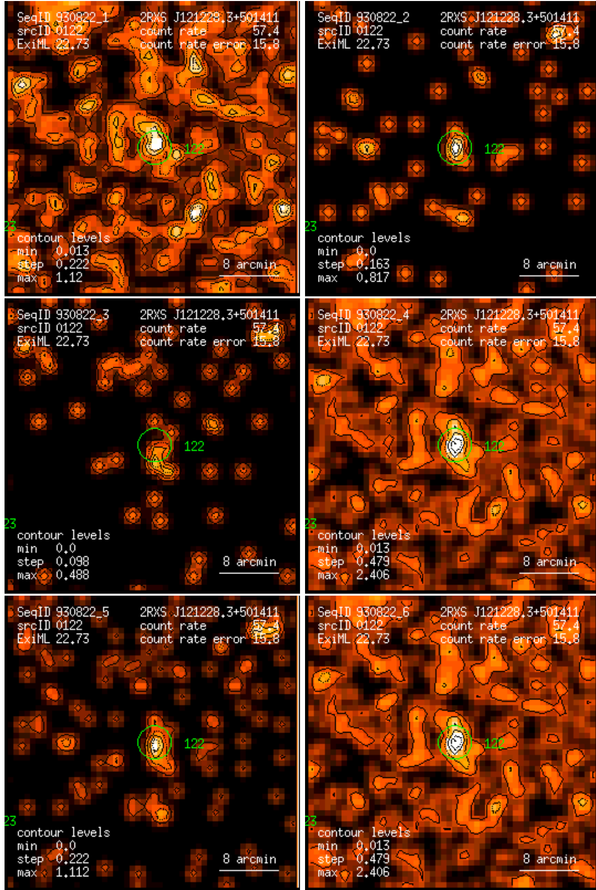
Figure 122: RASS 930822: detection 0122: band rate images, Gaussian filter: (1) PSPC channels 11 – 41, (2) 52 – 90, (3) 91 – 201, (4) 11 – 235, (5) 52 – 201, (6) 11 – 201. Broad band rates in counts/ks. Band rate contour levels in counts/ks/arcmin 2 .
