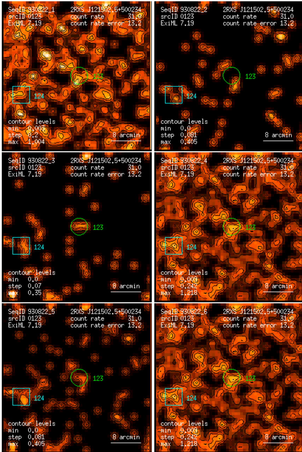
Figure 123: RASS 930822: detection 0123: band rate images, Gaussian filter: (1) PSPC channels 11 – 41, (2) 52 – 90, (3) 91 – 201, (4) 11 – 235, (5) 52 – 201, (6) 11 – 201. Broad band rates in counts/ks. Band rate contour levels in counts/ks/arcmin 2 .
