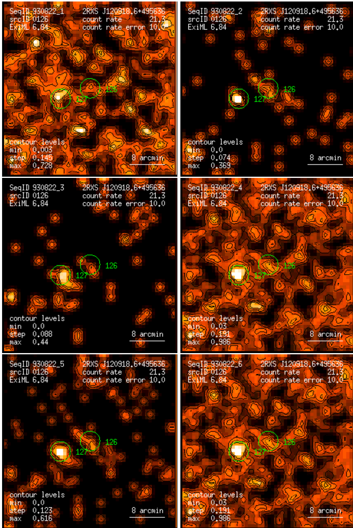
Figure 126: RASS 930822: detection 0126: band rate images, Gaussian filter: (1) PSPC channels 11 – 41, (2) 52 – 90, (3) 91 – 201, (4) 11 – 235, (5) 52 – 201, (6) 11 – 201. Broad band rates in counts/ks. Band rate contour levels in counts/ks/arcmin 2 .
