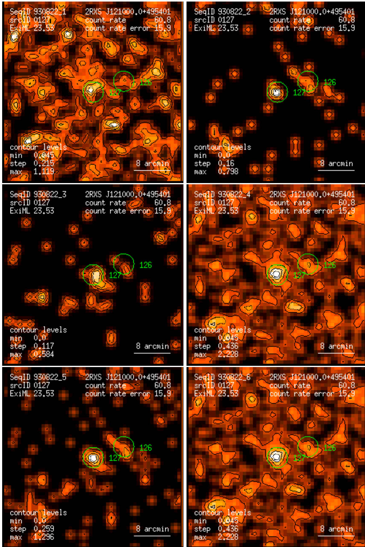
Figure 127: RASS 930822: detection 0127: band rate images, Gaussian filter: (1) PSPC channels 11 – 41, (2) 52 – 90, (3) 91 – 201, (4) 11 – 235, (5) 52 – 201, (6) 11 – 201. Broad band rates in counts/ks. Band rate contour levels in counts/ks/arcmin 2 .
