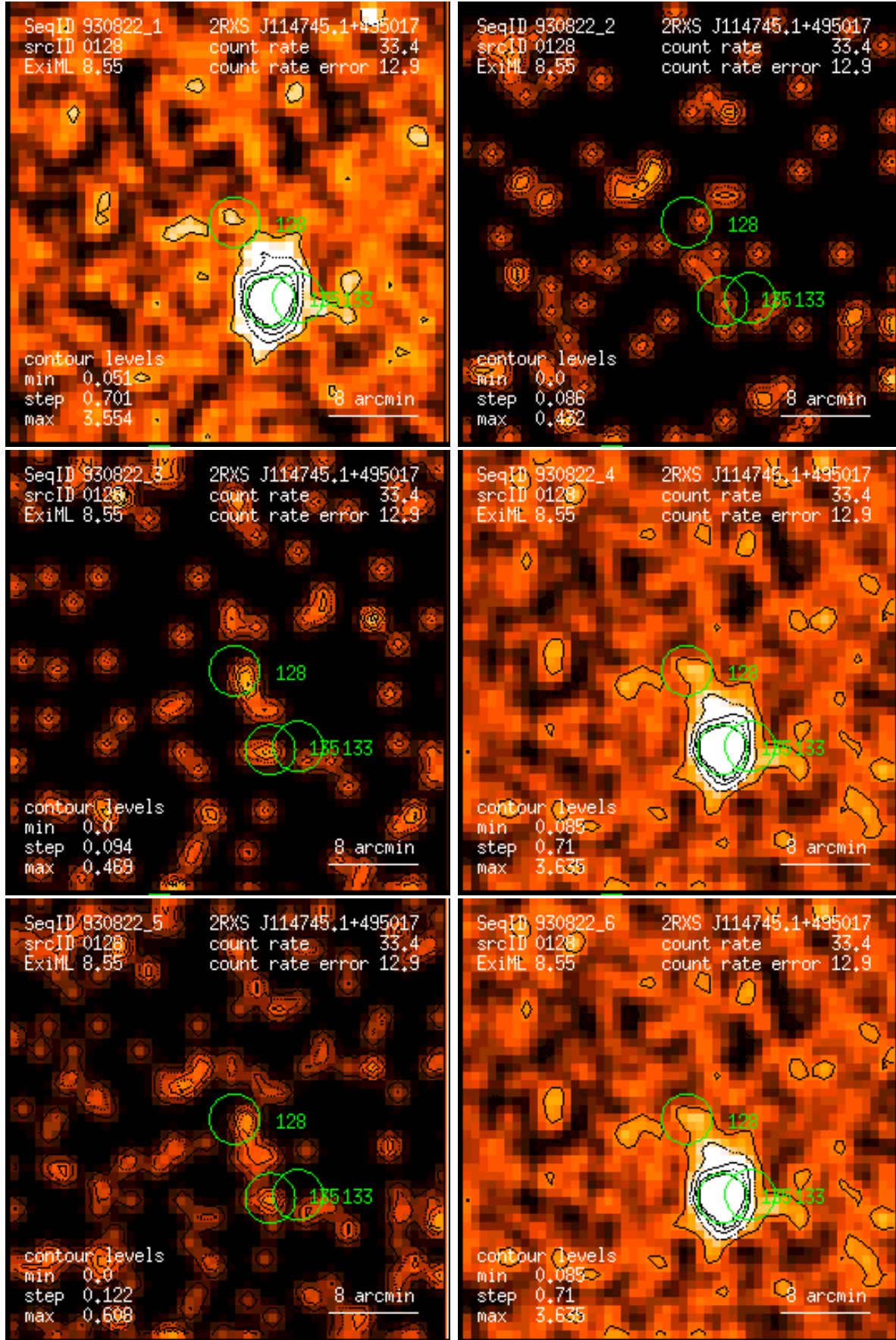
Figure 128: RASS 930822: detection 0128: band rate images, Gaussian filter: (1) PSPC channels 11 – 41, (2) 52 – 90, (3) 91 – 201, (4) 11 – 235, (5) 52 – 201, (6) 11 – 201. Broad band rates in counts/ks. Band rate contour levels in counts/ks/arcmin 2 .
