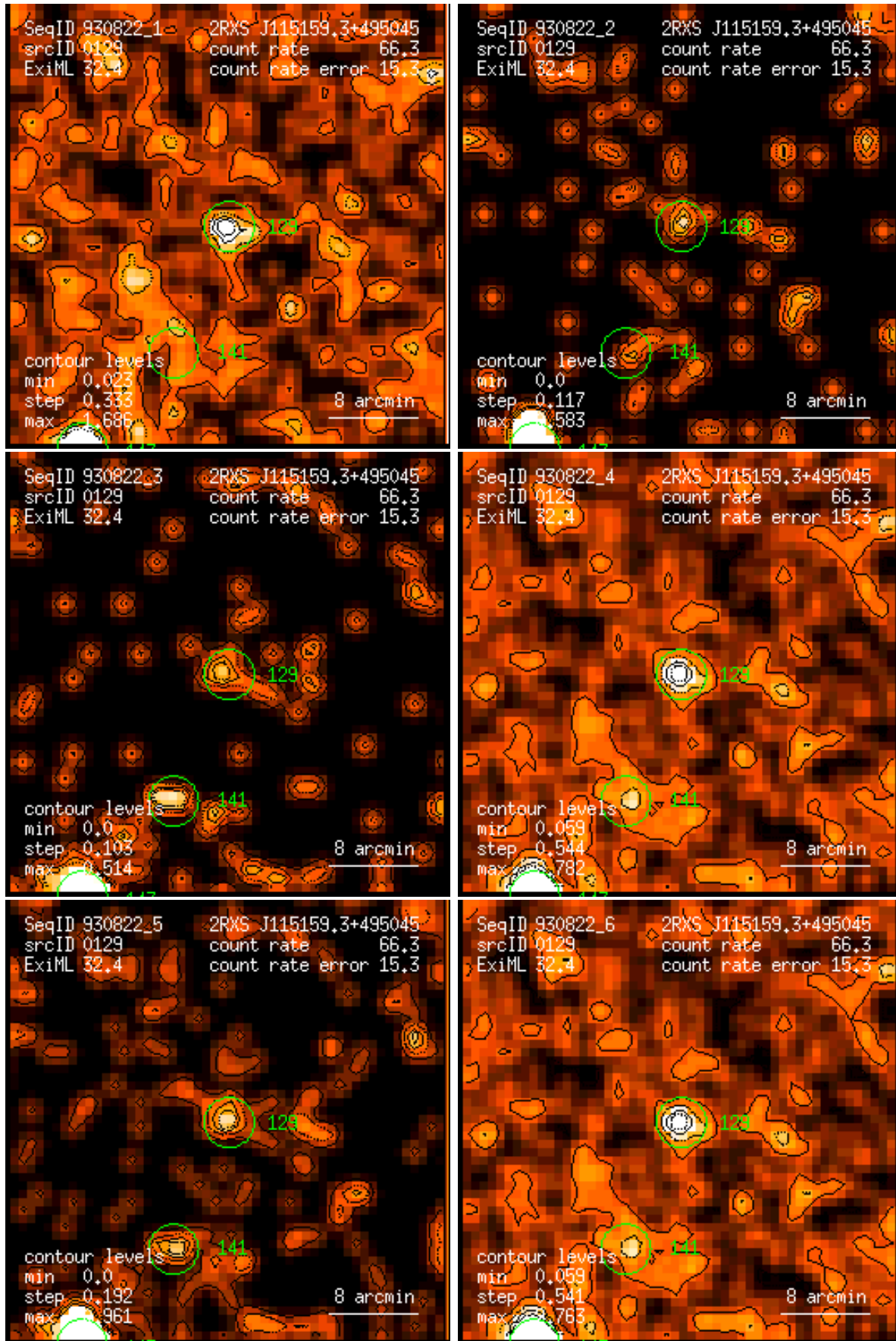
Figure 129: RASS 930822: detection 0129: band rate images, Gaussian filter: (1) PSPC channels 11 – 41, (2) 52 – 90, (3) 91 – 201, (4) 11 – 235, (5) 52 – 201, (6) 11 – 201. Broad band rates in counts/ks. Band rate contour levels in counts/ks/arcmin 2 .
