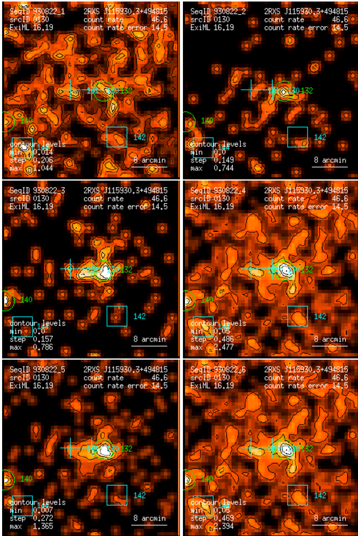
Figure 130: RASS 930822: detection 0130: band rate images, Gaussian filter: (1) PSPC channels 11 – 41, (2) 52 – 90, (3) 91 – 201, (4) 11 – 235, (5) 52 – 201, (6) 11 – 201. Broad band rates in counts/ks. Band rate contour levels in counts/ks/arcmin 2 .
