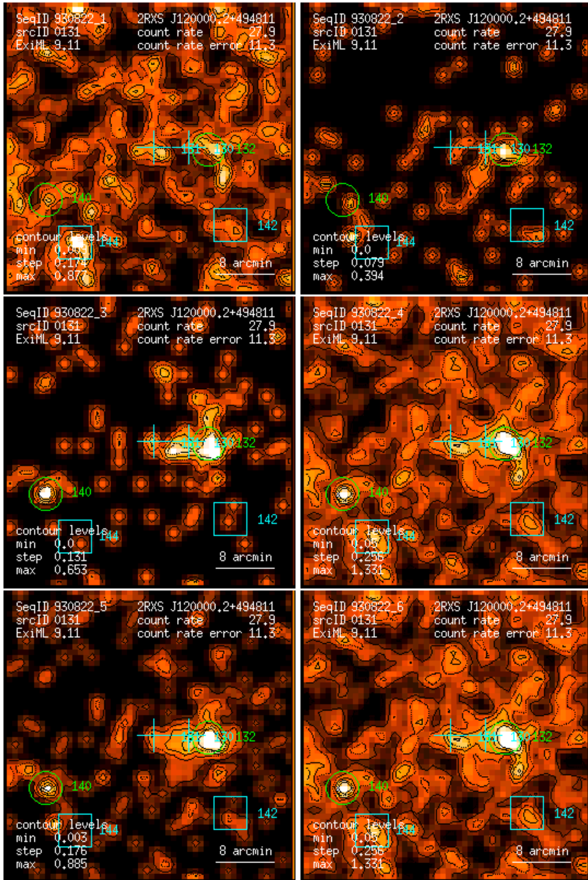
Figure 131: RASS 930822: detection 0131: band rate images, Gaussian filter: (1) PSPC channels 11 – 41, (2) 52 – 90, (3) 91 – 201, (4) 11 – 235, (5) 52 – 201, (6) 11 – 201. Broad band rates in counts/ks. Band rate contour levels in counts/ks/arcmin 2 .
