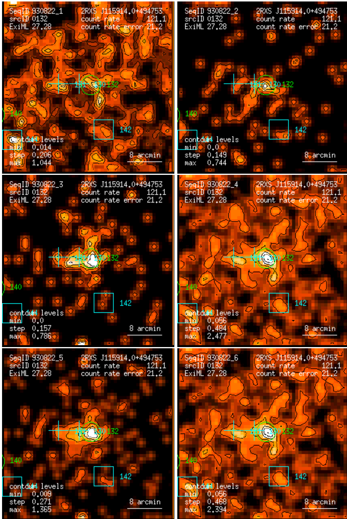
Figure 132: RASS 930822: detection 0132: band rate images, Gaussian filter: (1) PSPC channels 11 – 41, (2) 52 – 90, (3) 91 – 201, (4) 11 – 235, (5) 52 – 201, (6) 11 – 201. Broad band rates in counts/ks. Band rate contour levels in counts/ks/arcmin 2 .
