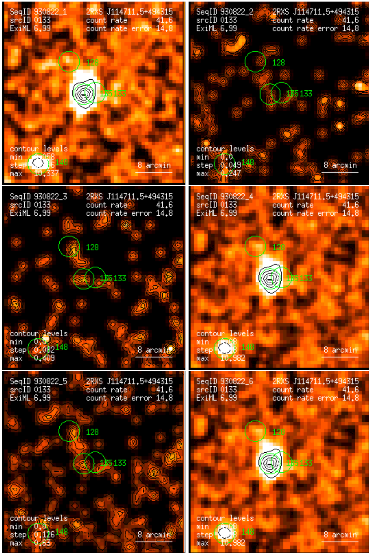
Figure 133: RASS 930822: detection 0133: band rate images, Gaussian filter: (1) PSPC channels 11 – 41, (2) 52 – 90, (3) 91 – 201, (4) 11 – 235, (5) 52 – 201, (6) 11 – 201. Broad band rates in counts/ks. Band rate contour levels in counts/ks/arcmin 2 .
