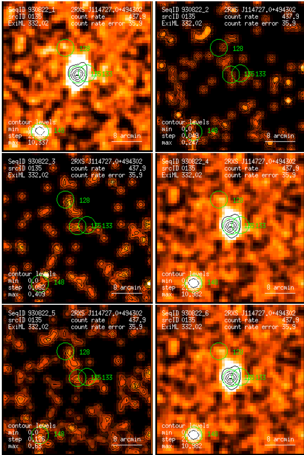
Figure 135: RASS 930822: detection 0135: band rate images, Gaussian filter: (1) PSPC channels 11 – 41, (2) 52 – 90, (3) 91 – 201, (4) 11 – 235, (5) 52 – 201, (6) 11 – 201. Broad band rates in counts/ks. Band rate contour levels in counts/ks/arcmin 2 .
