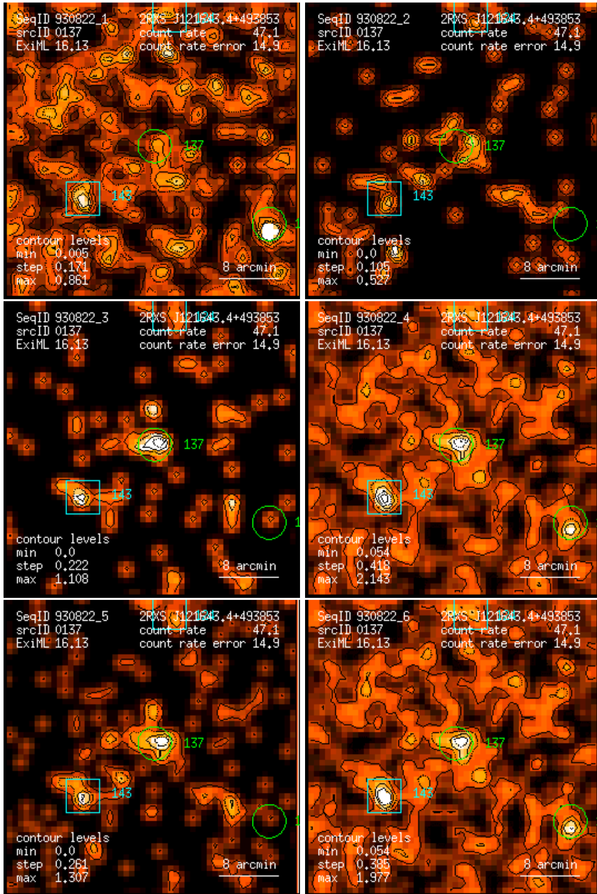
Figure 137: RASS 930822: detection 0137: band rate images, Gaussian filter: (1) PSPC channels 11 – 41, (2) 52 – 90, (3) 91 – 201, (4) 11 – 235, (5) 52 – 201, (6) 11 – 201. Broad band rates in counts/ks. Band rate contour levels in counts/ks/arcmin 2 .
