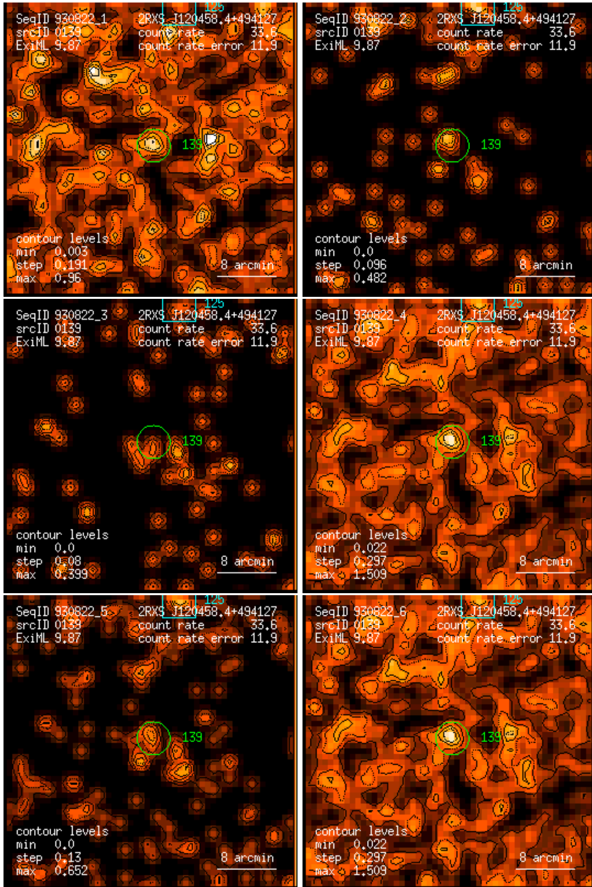
Figure 139: RASS 930822: detection 0139: band rate images, Gaussian filter: (1) PSPC channels 11 – 41, (2) 52 – 90, (3) 91 – 201, (4) 11 – 235, (5) 52 – 201, (6) 11 – 201. Broad band rates in counts/ks. Band rate contour levels in counts/ks/arcmin 2 .
