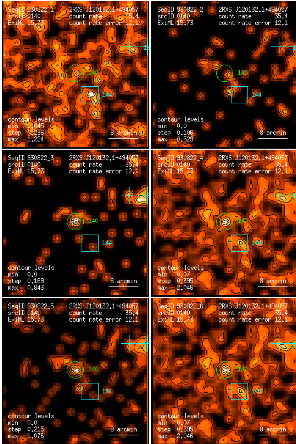
Figure 140: RASS 930822: detection 0140: band rate images, Gaussian filter: (1) PSPC channels 11 – 41, (2) 52 – 90, (3) 91 – 201, (4) 11 – 235, (5) 52 – 201, (6) 11 – 201. Broad band rates in counts/ks. Band rate contour levels in counts/ks/arcmin 2 .
