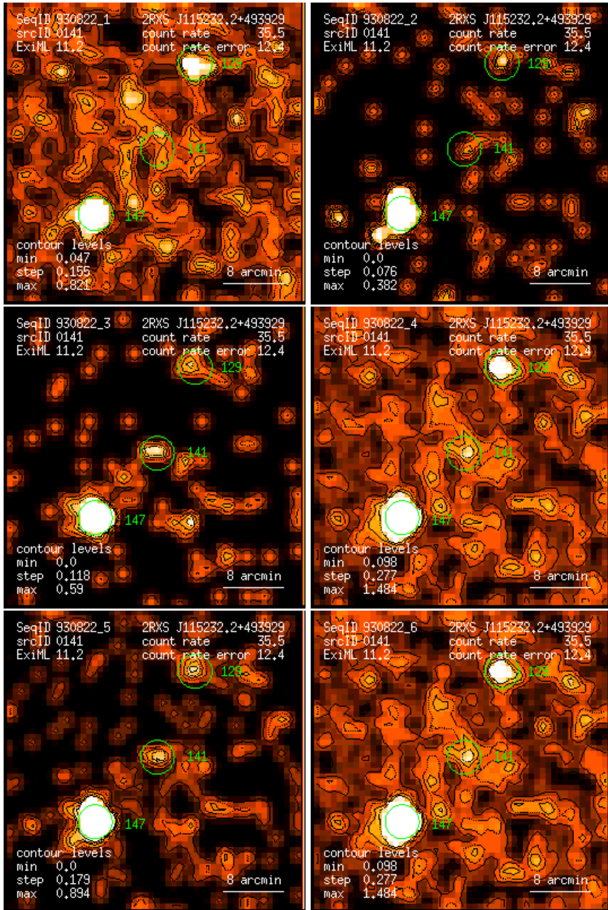
Figure 141: RASS 930822: detection 0141: band rate images, Gaussian filter: (1) PSPC channels 11 – 41, (2) 52 – 90, (3) 91 – 201, (4) 11 – 235, (5) 52 – 201, (6) 11 – 201. Broad band rates in counts/ks. Band rate contour levels in counts/ks/arcmin 2 .
