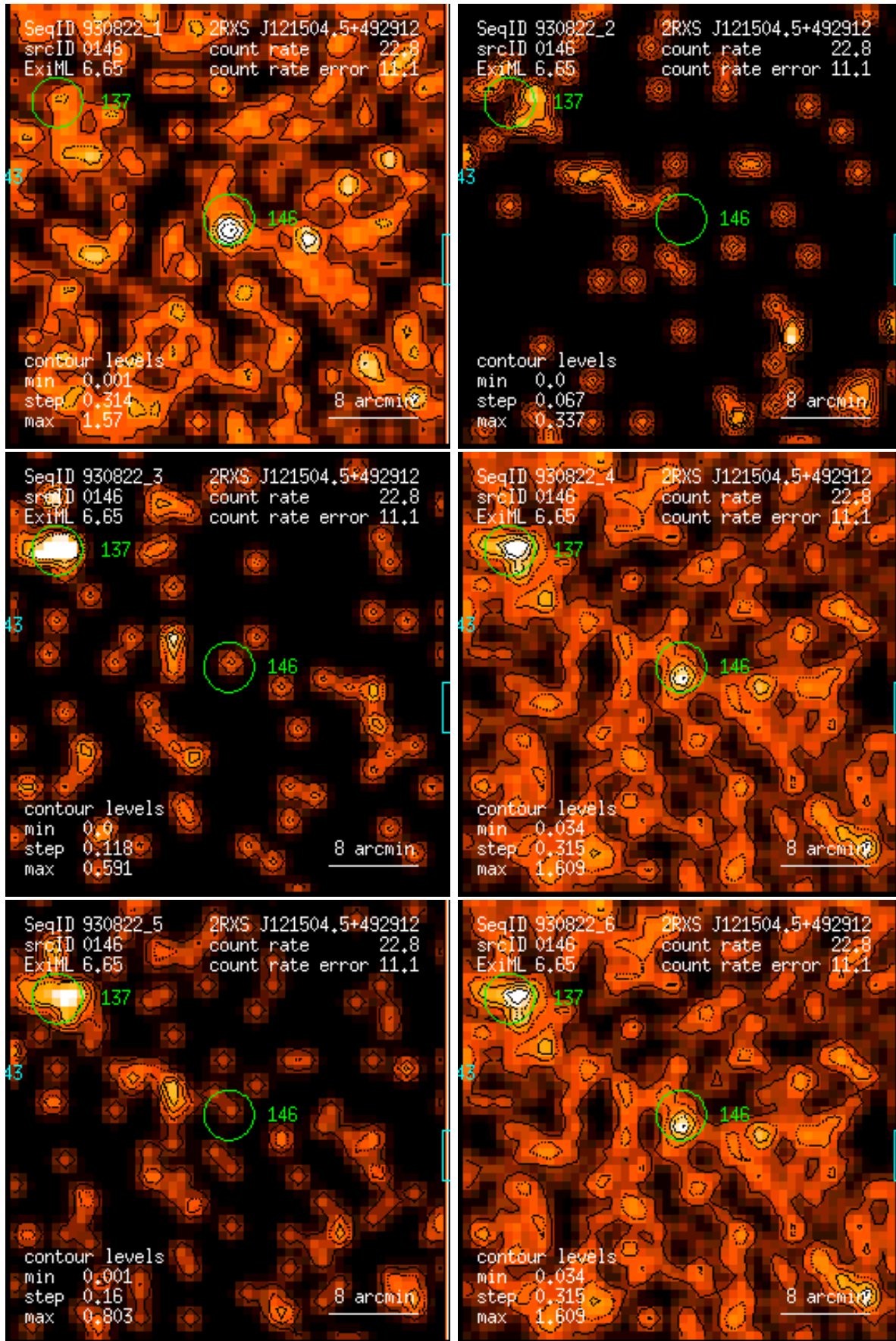
Figure 146: RASS 930822: detection 0146: band rate images, Gaussian filter: (1) PSPC channels 11 – 41, (2) 52 – 90, (3) 91 – 201, (4) 11 – 235, (5) 52 – 201, (6) 11 – 201. Broad band rates in counts/ks. Band rate contour levels in counts/ks/arcmin 2 .
