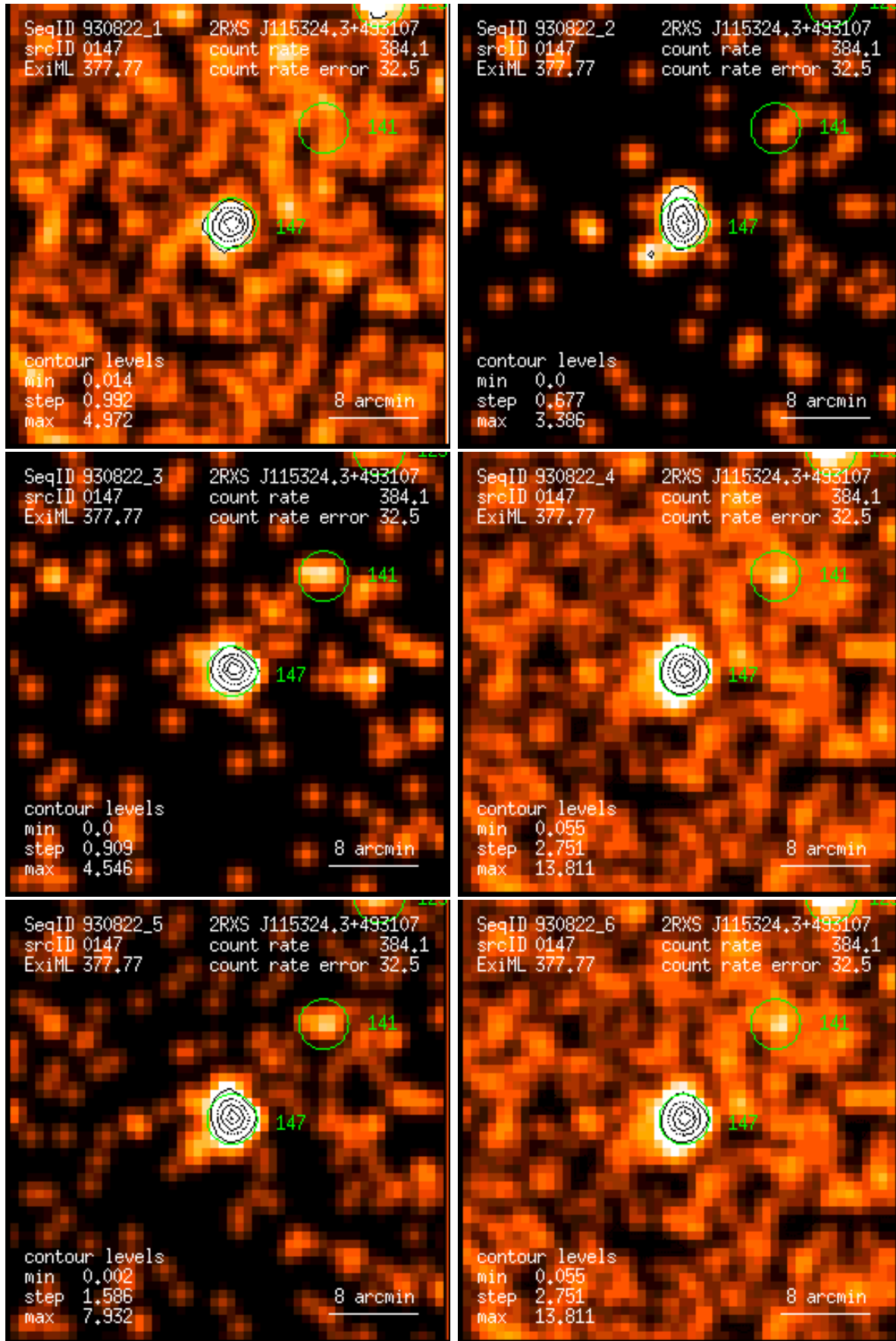
Figure 147: RASS 930822: detection 0147: band rate images, Gaussian filter: (1) PSPC channels 11 – 41, (2) 52 – 90, (3) 91 – 201, (4) 11 – 235, (5) 52 – 201, (6) 11 – 201. Broad band rates in counts/ks. Band rate contour levels in counts/ks/arcmin 2 .
