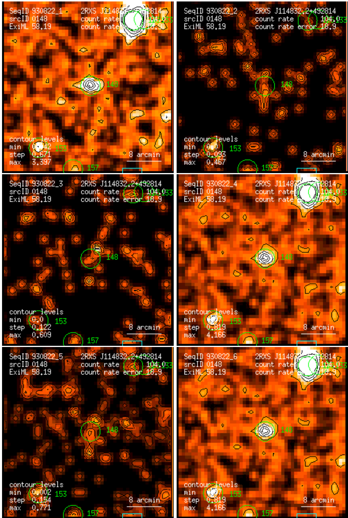
Figure 148: RASS 930822: detection 0148: band rate images, Gaussian filter: (1) PSPC channels 11 – 41, (2) 52 – 90, (3) 91 – 201, (4) 11 – 235, (5) 52 – 201, (6) 11 – 201. Broad band rates in counts/ks. Band rate contour levels in counts/ks/arcmin 2 .
