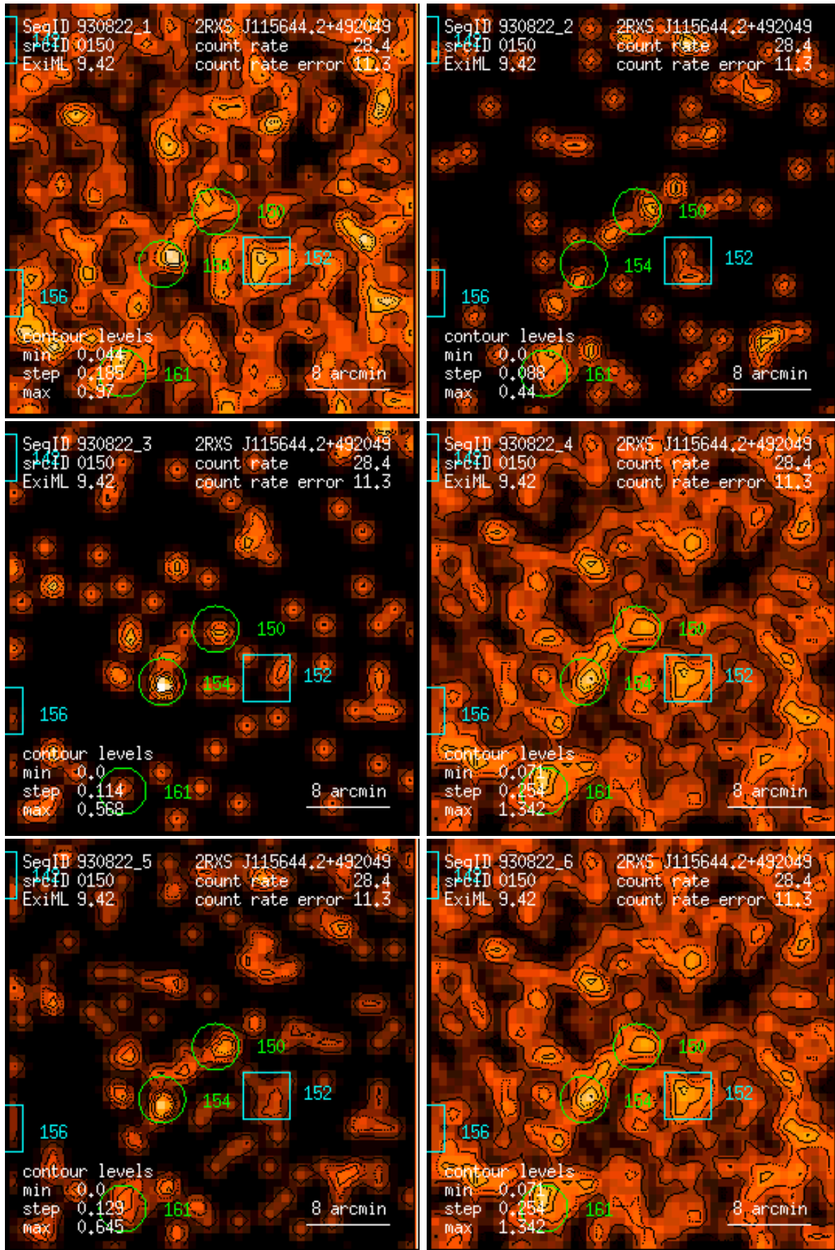
Figure 150: RASS 930822: detection 0150: band rate images, Gaussian filter: (1) PSPC channels 11 – 41, (2) 52 – 90, (3) 91 – 201, (4) 11 – 235, (5) 52 – 201, (6) 11 – 201. Broad band rates in counts/ks. Band rate contour levels in counts/ks/arcmin 2 .
