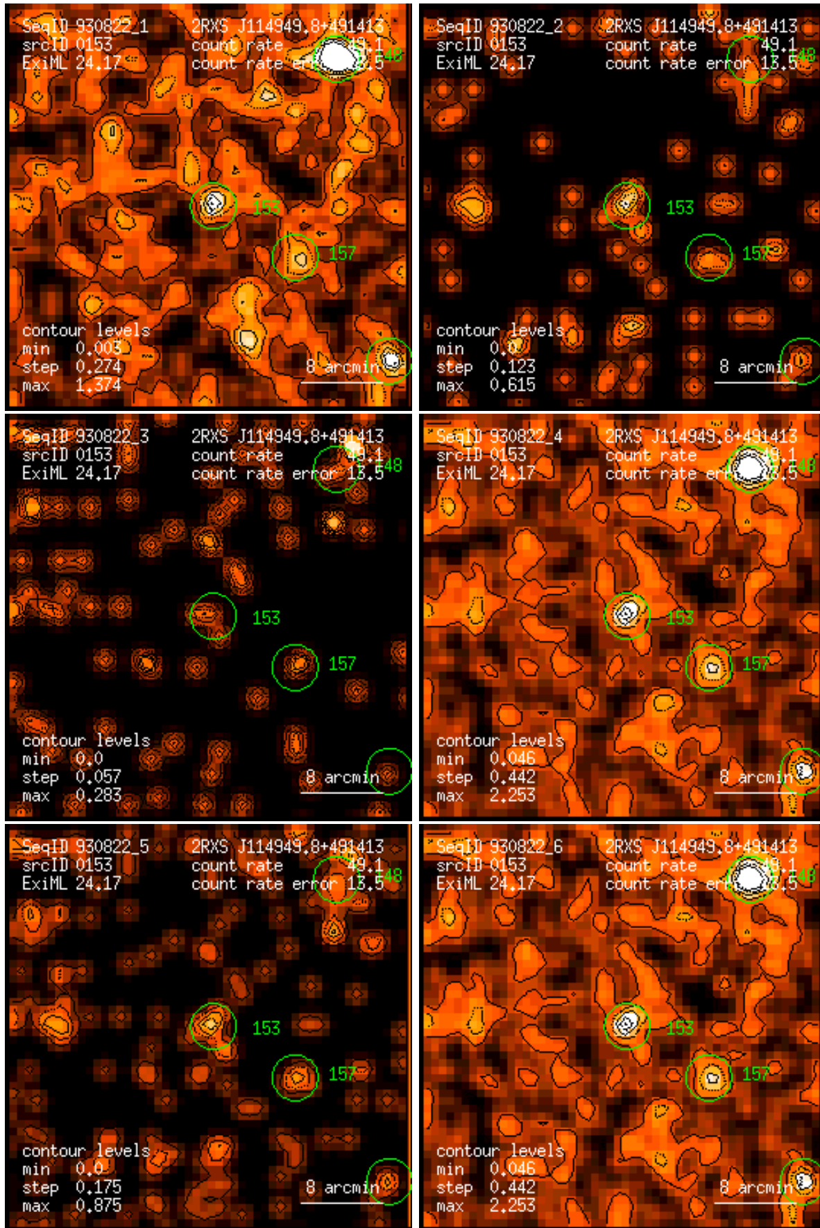
Figure 153: RASS 930822: detection 0153: band rate images, Gaussian filter: (1) PSPC channels 11 – 41, (2) 52 – 90, (3) 91 – 201, (4) 11 – 235, (5) 52 – 201, (6) 11 – 201. Broad band rates in counts/ks. Band rate contour levels in counts/ks/arcmin 2 .
