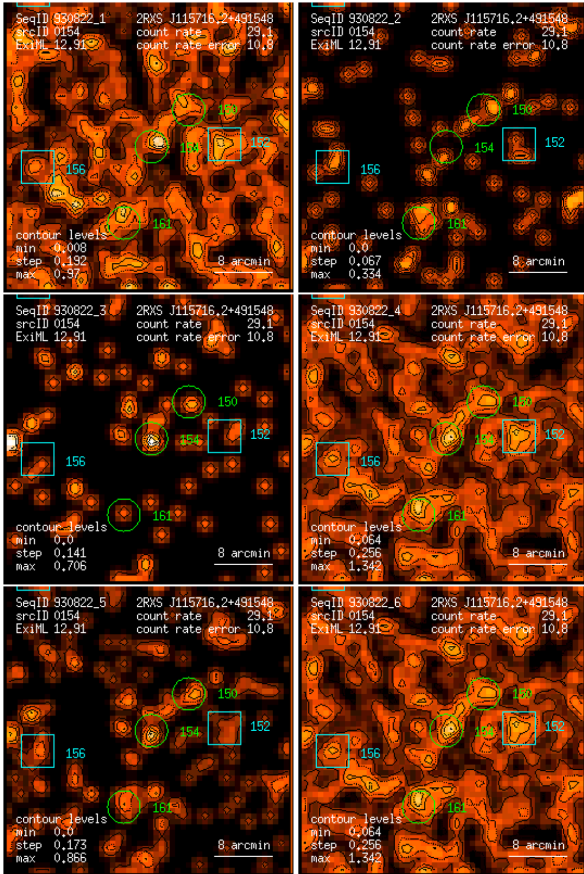
Figure 154: RASS 930822: detection 0154: band rate images, Gaussian filter: (1) PSPC channels 11 – 41, (2) 52 – 90, (3) 91 – 201, (4) 11 – 235, (5) 52 – 201, (6) 11 – 201. Broad band rates in counts/ks. Band rate contour levels in counts/ks/arcmin 2 .
