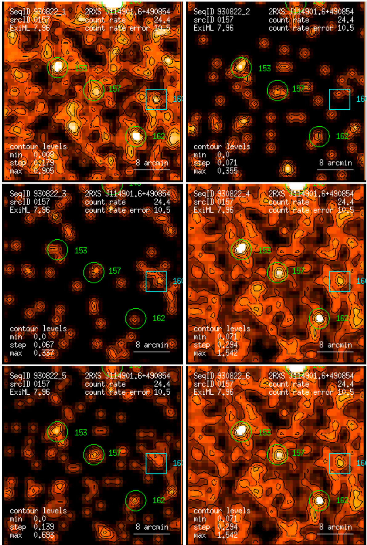
Figure 157: RASS 930822: detection 0157: band rate images, Gaussian filter: (1) PSPC channels 11 – 41, (2) 52 – 90, (3) 91 – 201, (4) 11 – 235, (5) 52 – 201, (6) 11 – 201. Broad band rates in counts/ks. Band rate contour levels in counts/ks/arcmin 2 .
